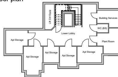
Floor plan
