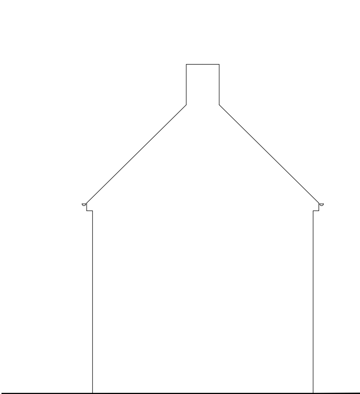
EXISTING SIDE ELEVATIONS
