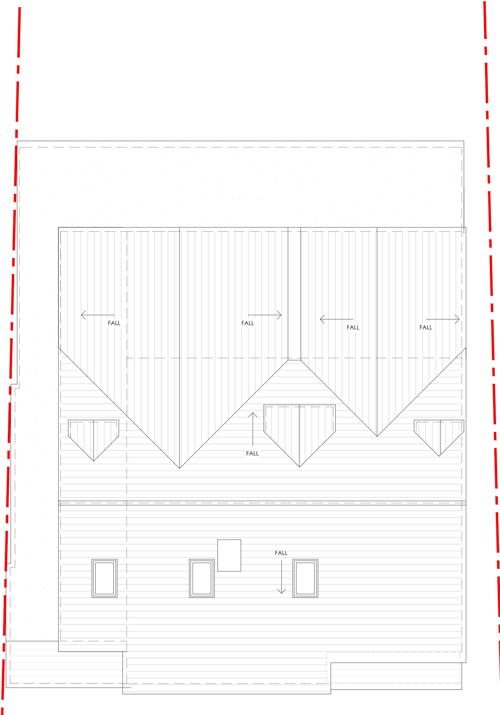
PROPOSED Roof Plan scale 1:50 @ A1
