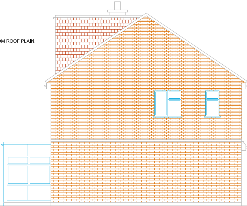
PROPOSED SIDE ELEVATION-2
