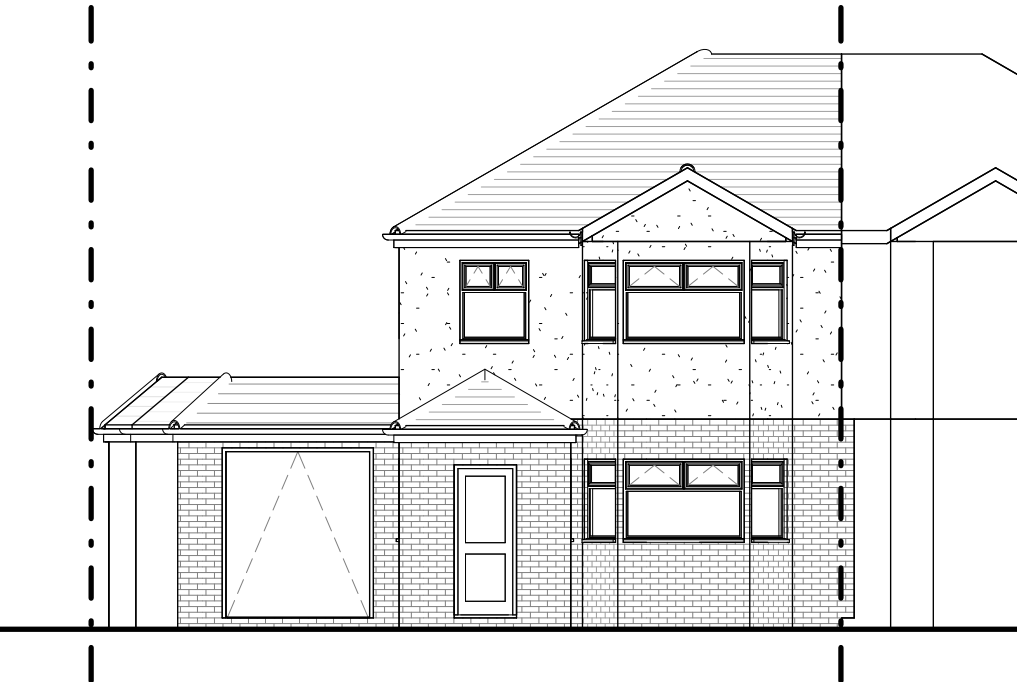
1 EXISTING SOUTH ELEVATION.
