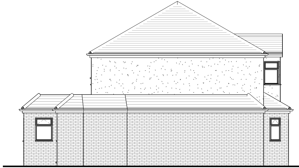
2 EXISTING WEST ELEVATION.
