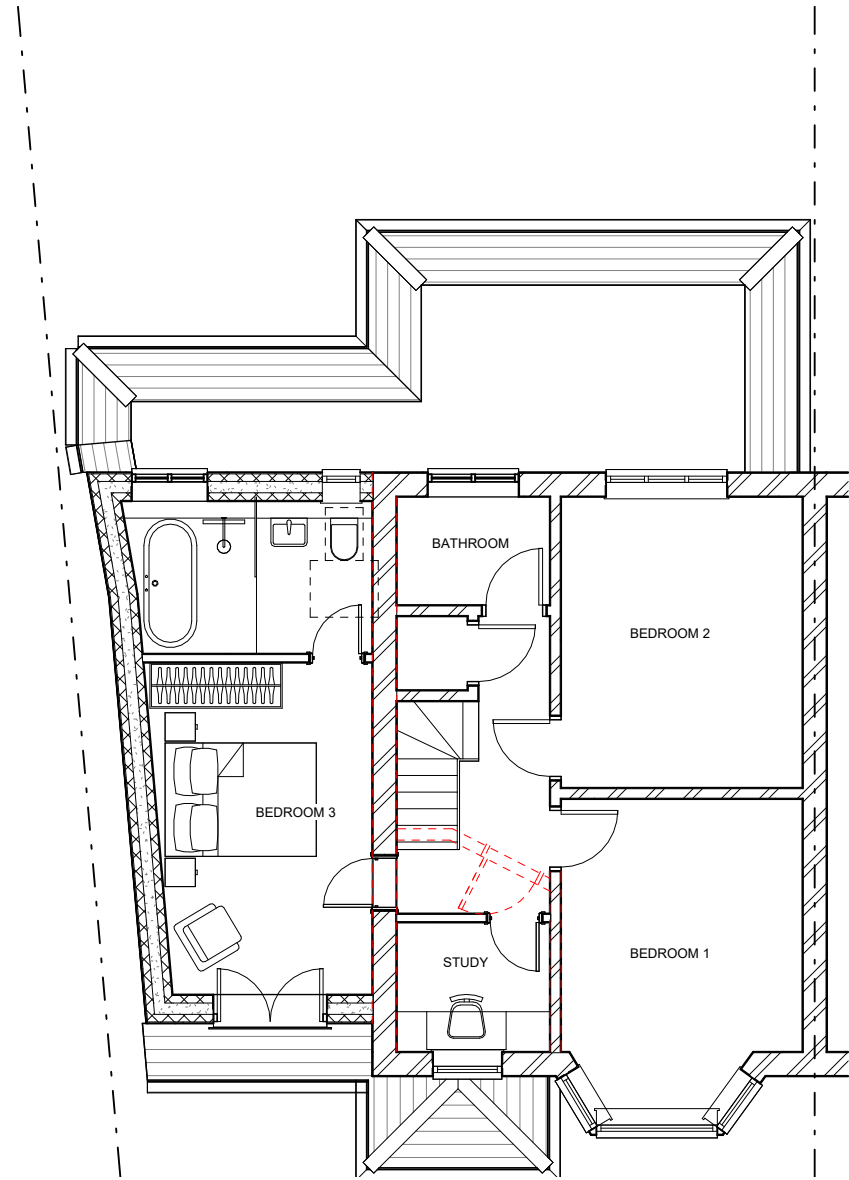
1 PROPOSED FIRST FLOOR PLAN.
