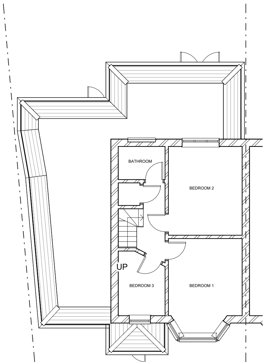
1 EXISTING FIRST FLOOR PLAN.
