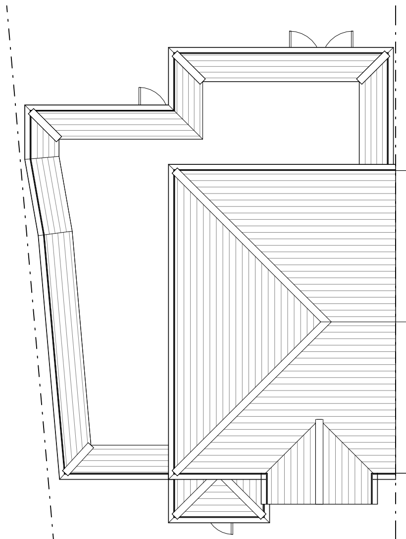
2 EXISTING ROOF PLAN.
