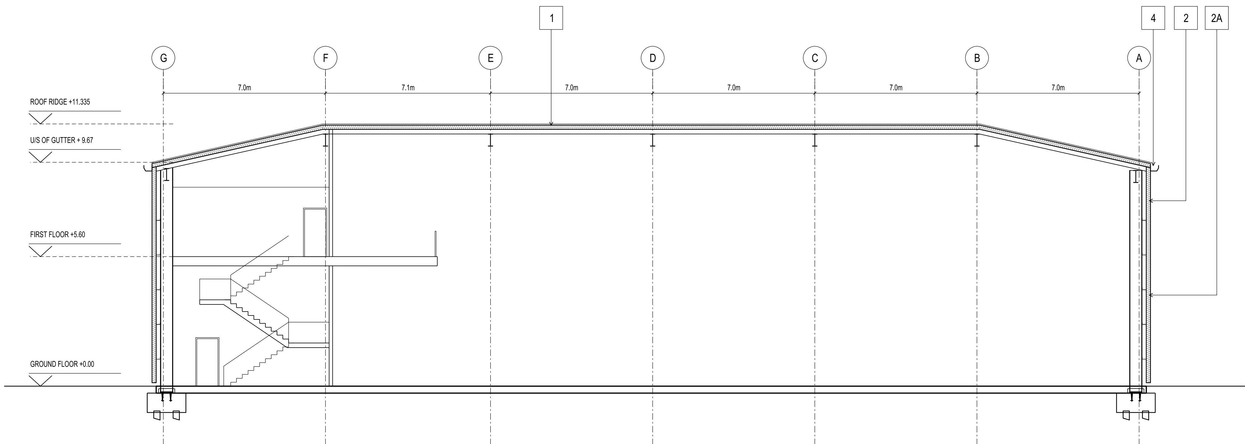
PROPOSED SECTION BB
