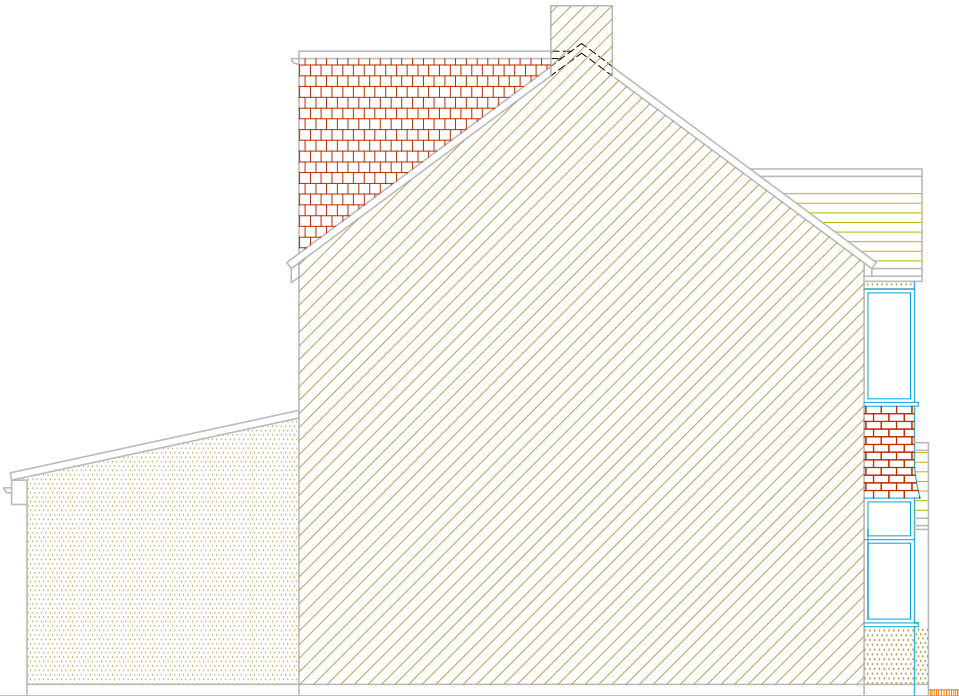
PRE-EXISTING SIDE ELEVATION-1
