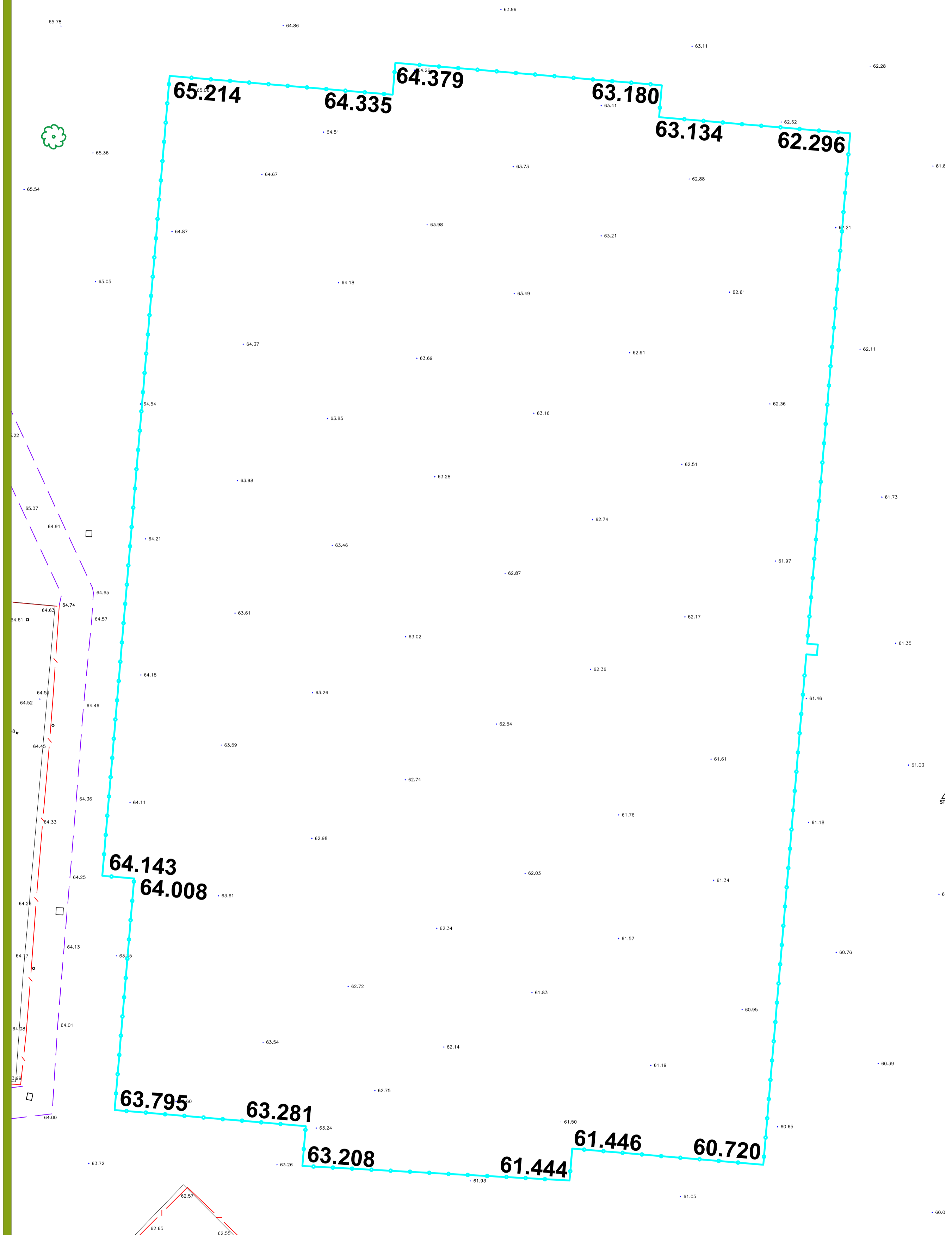
Existing Site Levels
