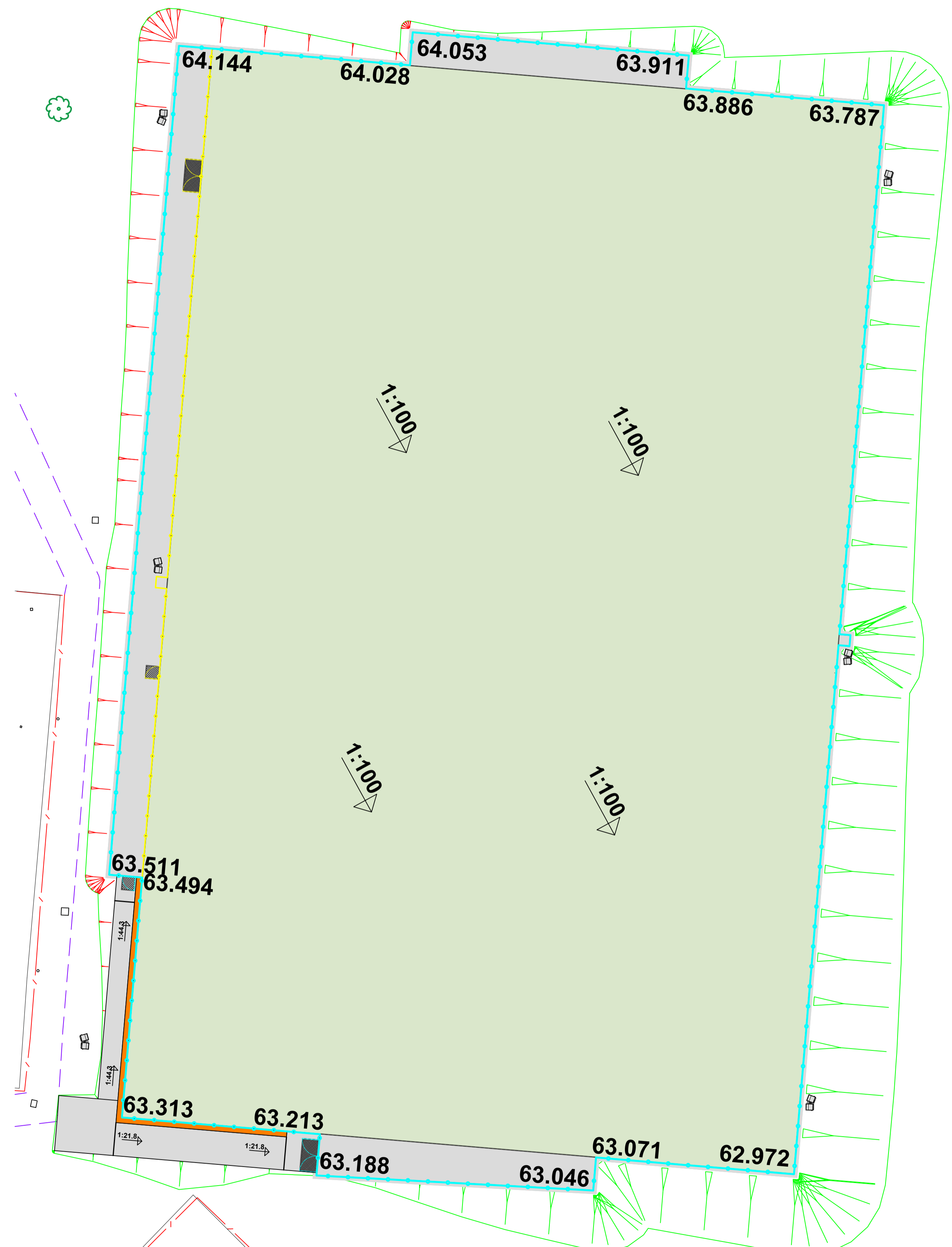
Proposed Site Levels
