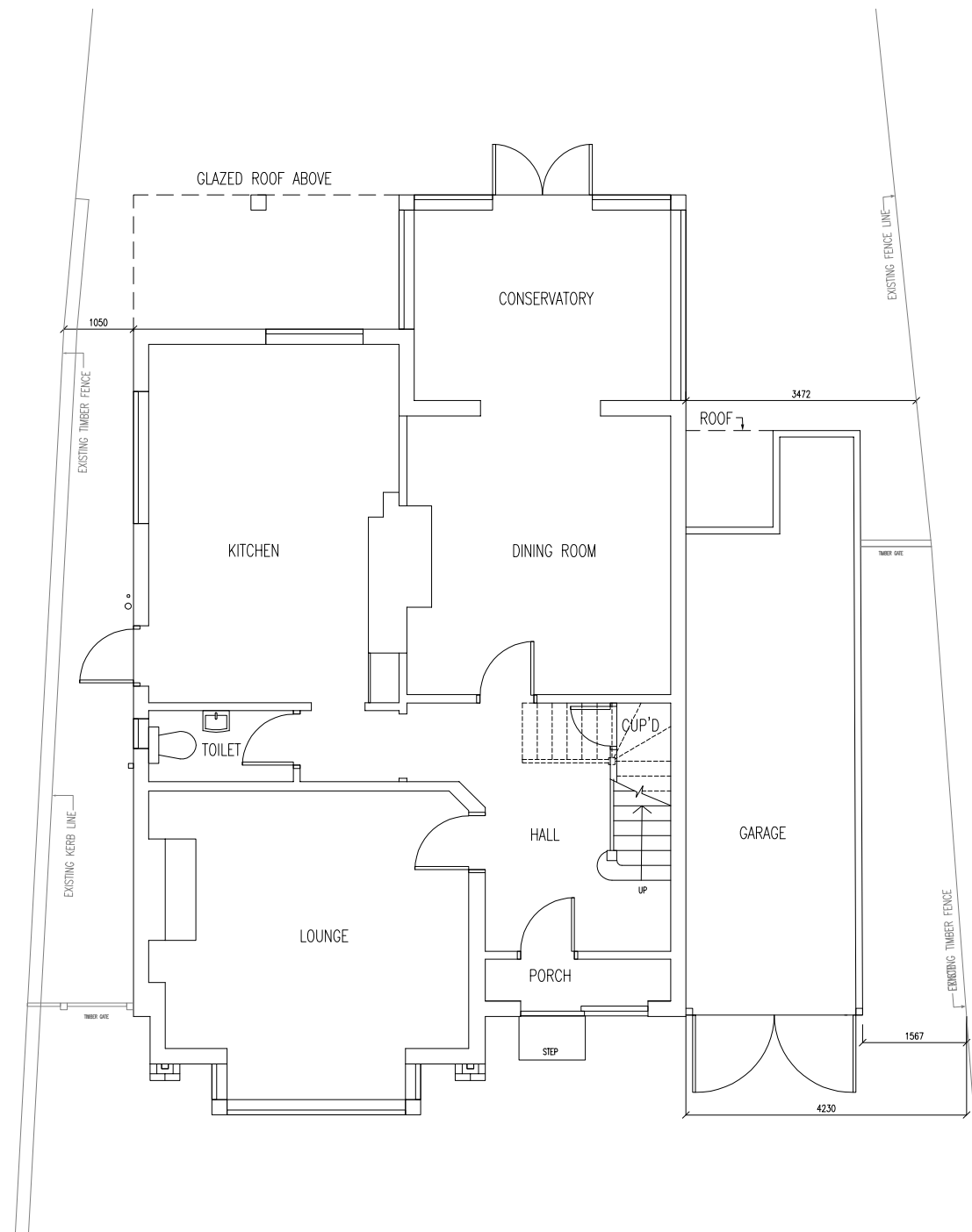
GROUND FLOOR
