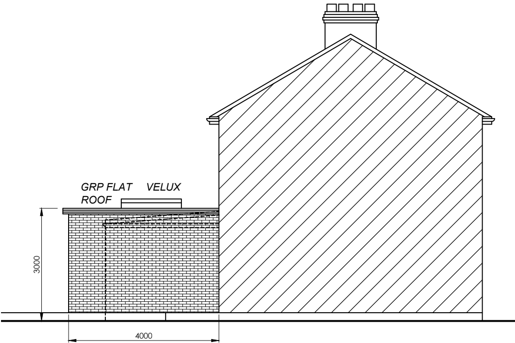
PROP OTHER SIDE ELEVATION
