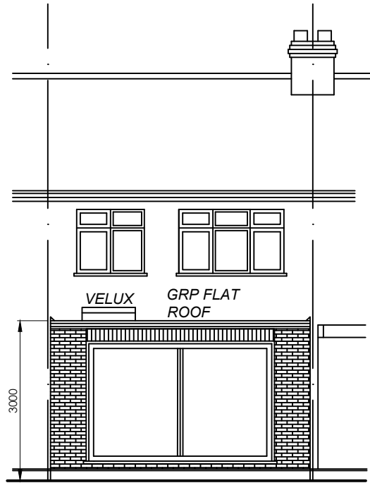
PROP REAR ELEVATION
