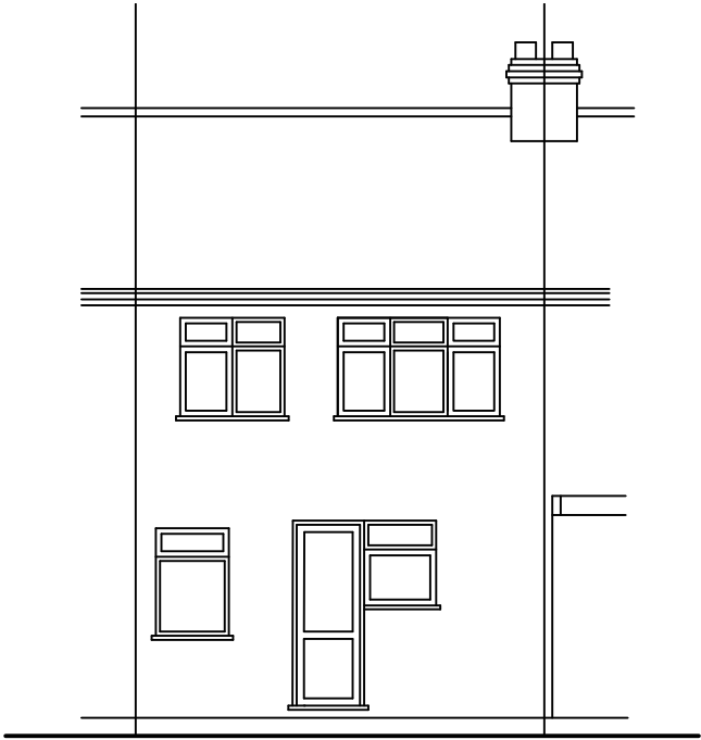
EXTG REAR ELEVATION
