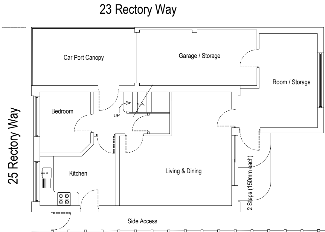
GROUND FLOOR PLAN (Existing)
