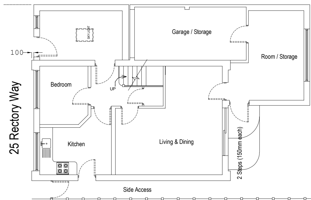
GROUND FLOOR PLAN (Proposed)
