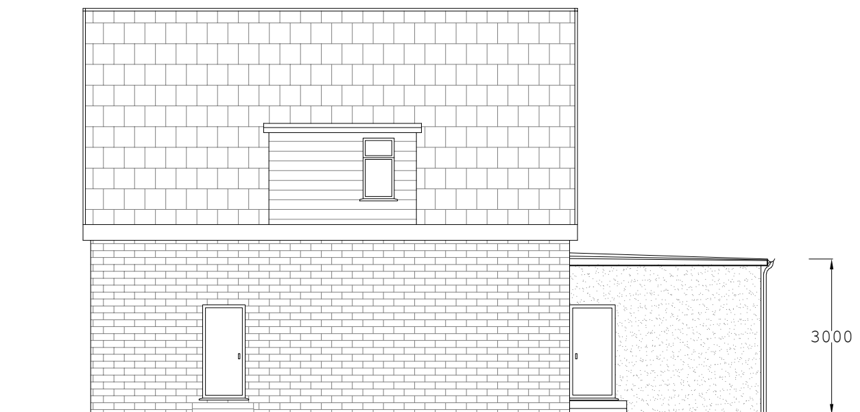
LEFT SIDE ELEVATION (Existing)
