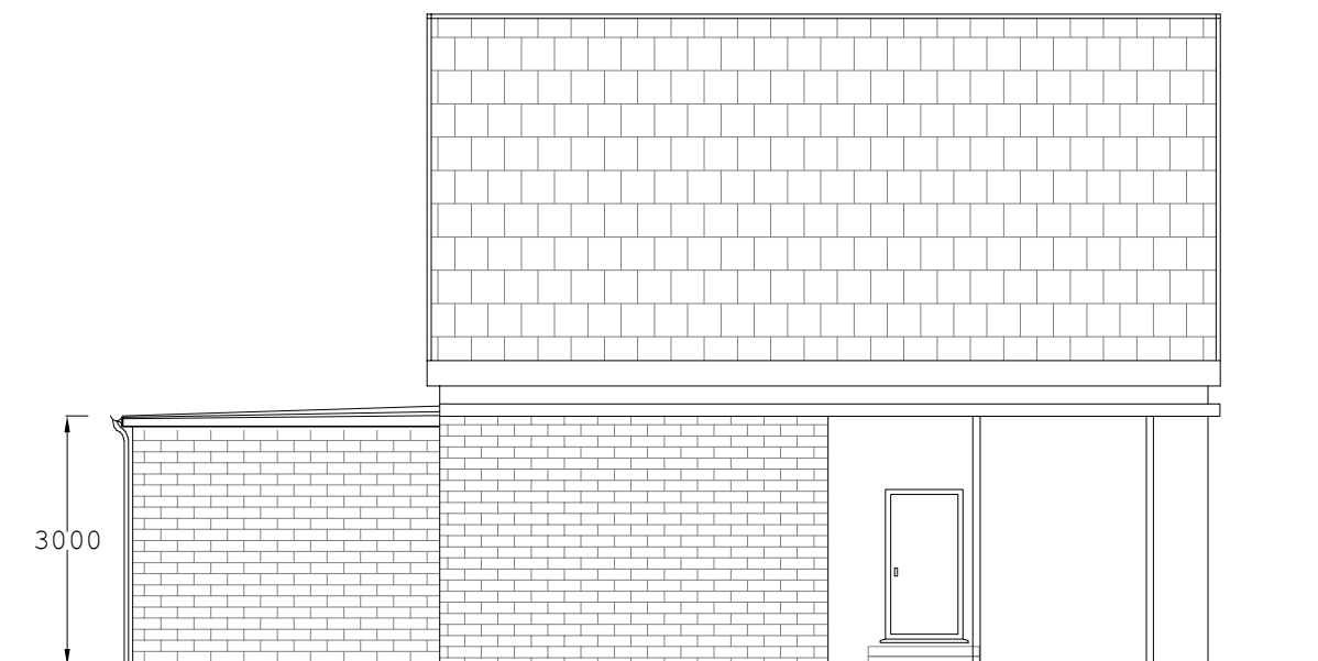
RIGHT SIDE ELEVATION (Existing)
