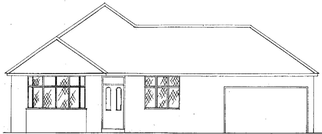
Front Elevation
