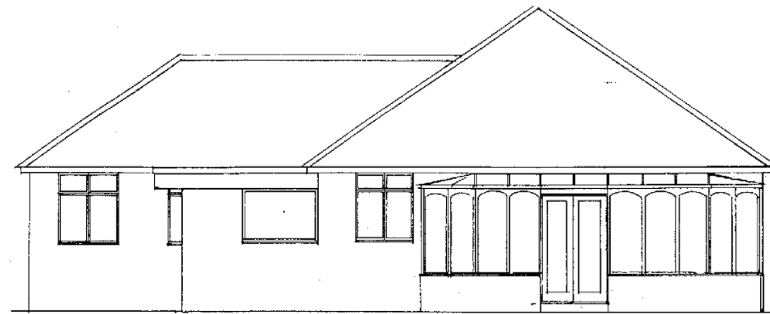
Rear Elevation
