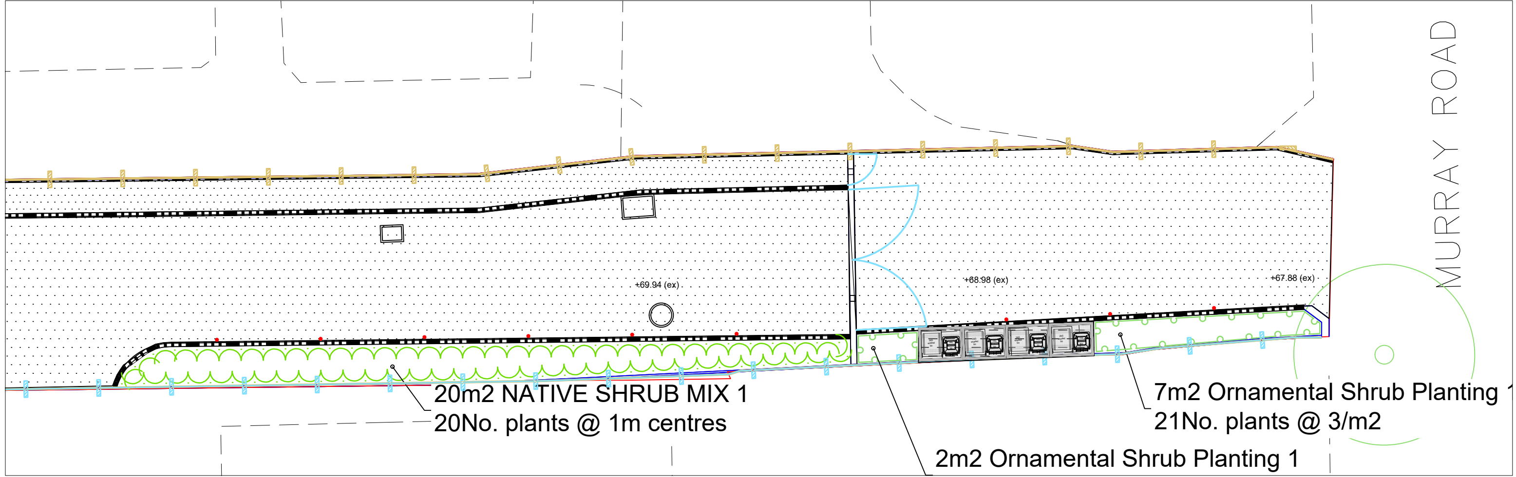
Plant Schedule
