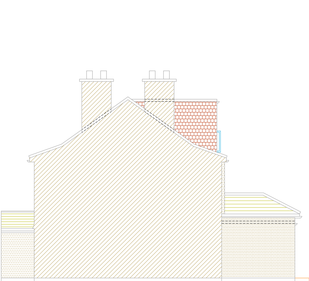
EXISTING SIDE ELEVATION-1
