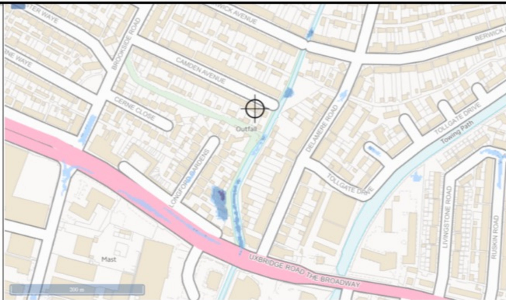
Figure 6 Environment Agency's Surface Water Flood Depth Map
