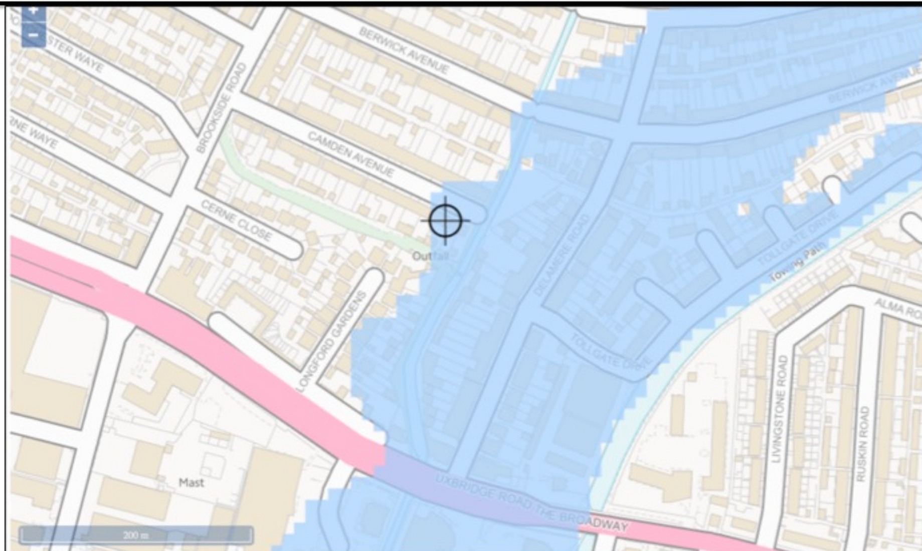
Figure 7 Environment Agency's Reservoir Flood Risk Map
