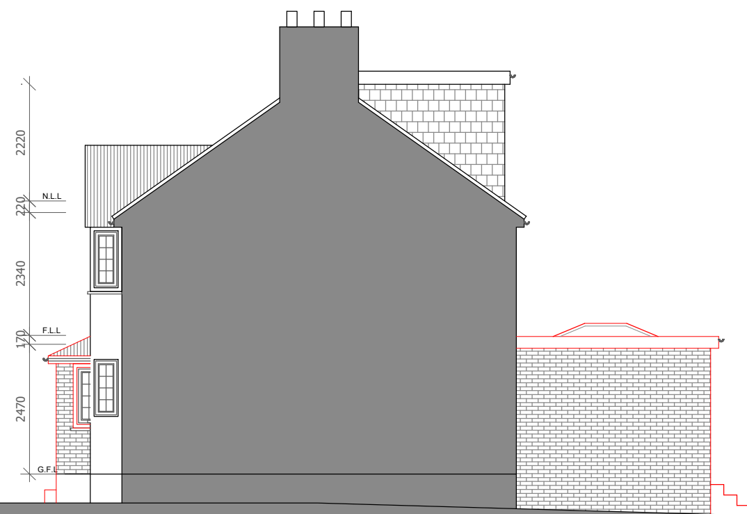
PROPOSED SIDE SECTIONAL ELEVATION
