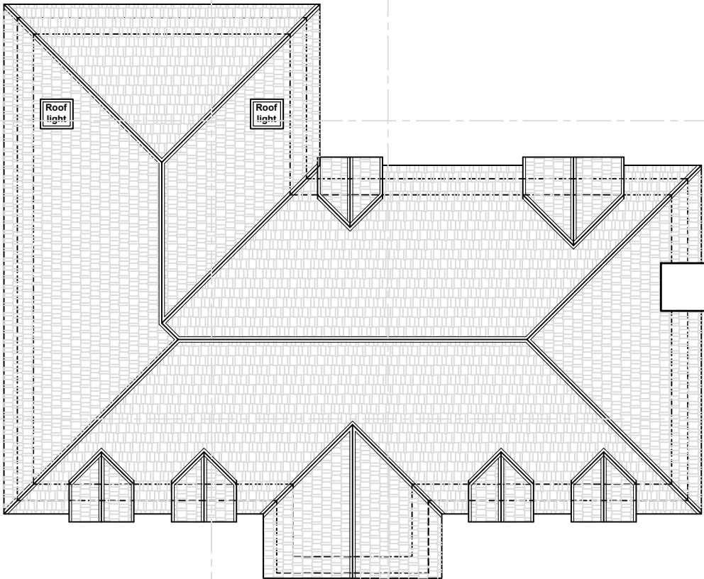
ROOF PLAN
