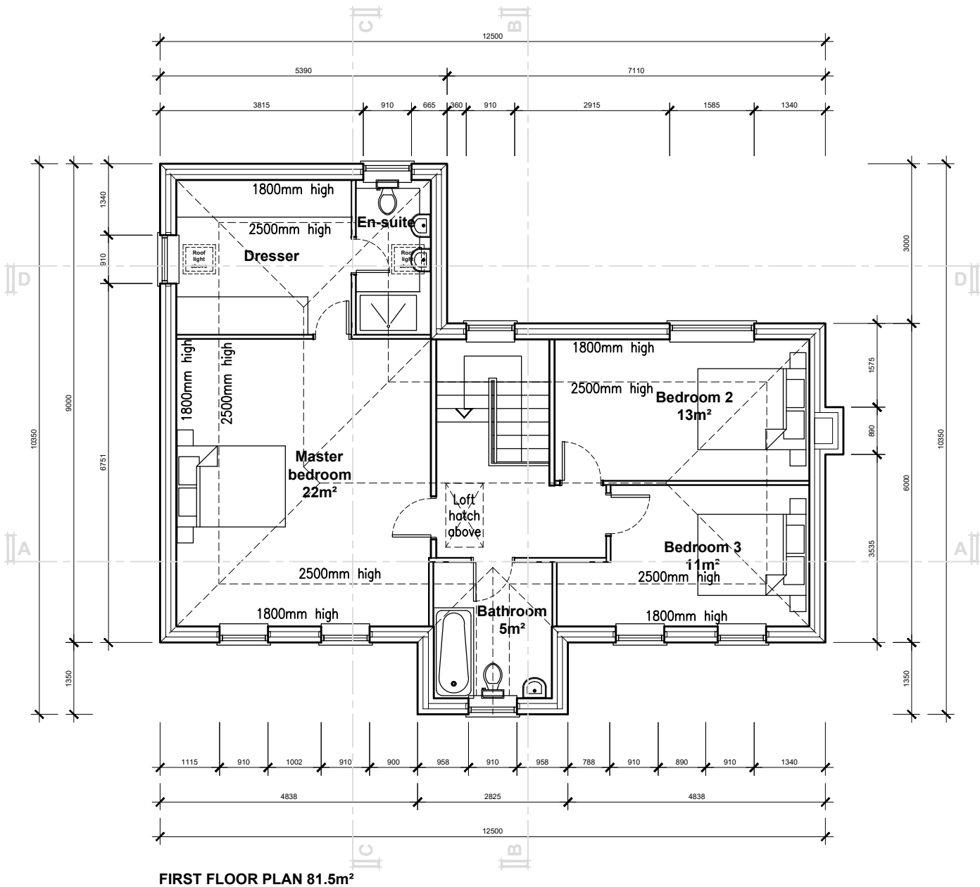
FIRST FLOOR PLAN 81.5m²
