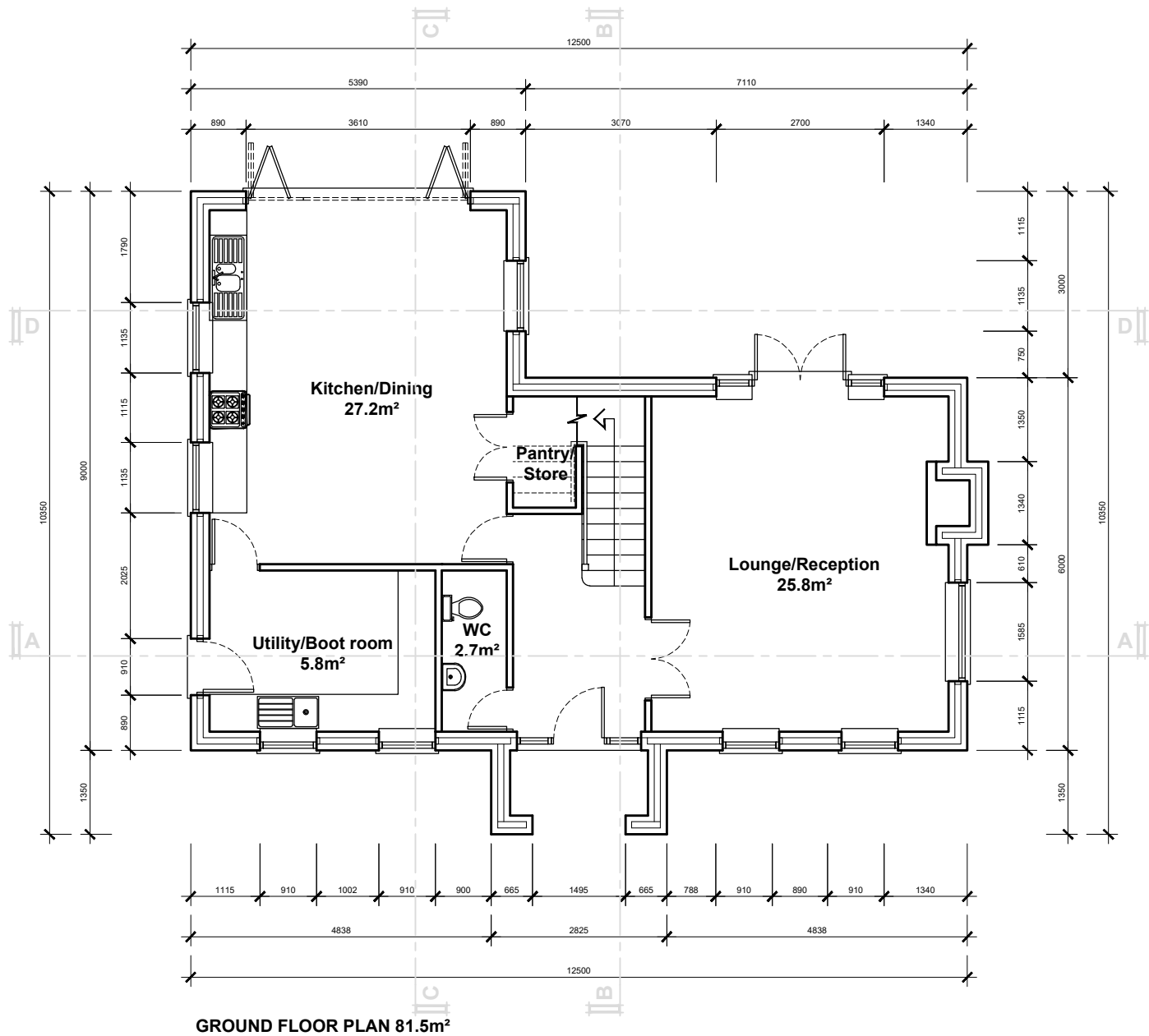
GROUND FLOOR PLAN 81.5m²
