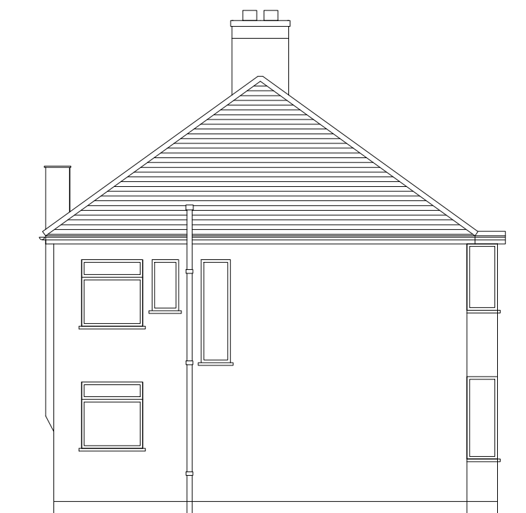
PRE EXISTING SIDE ELEVATION
