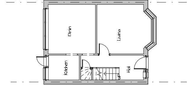
Ground Floor - Existing 1 : 100
