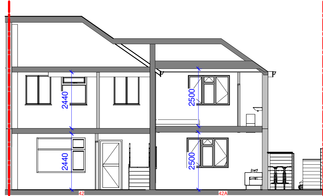
2 PROPOSED SECTION 1 : 100
