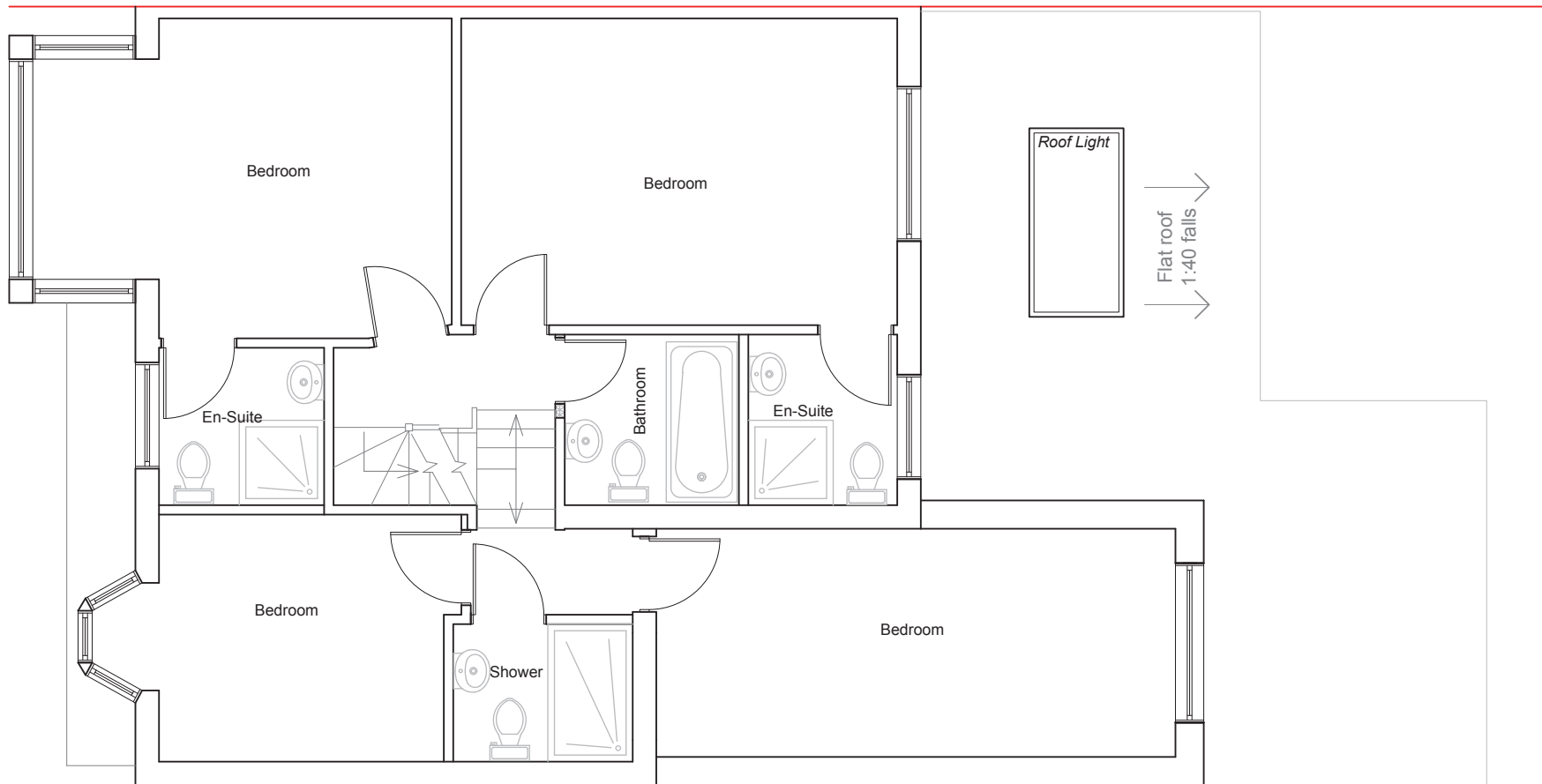
PROPOSED FIRST FLOOR PLAN 1:50
