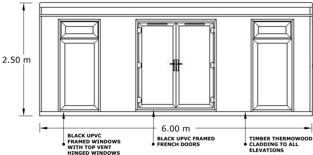
REAR ELEVATION
