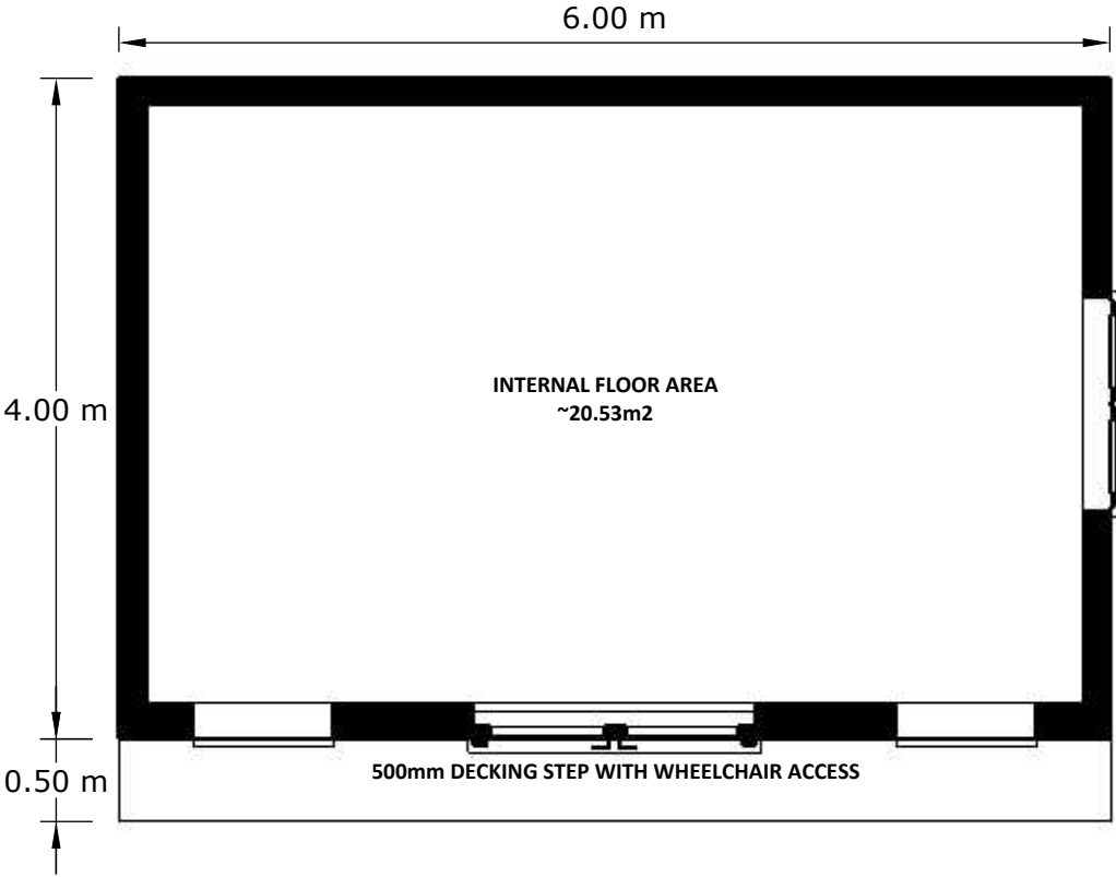
FLOOR PLAN
