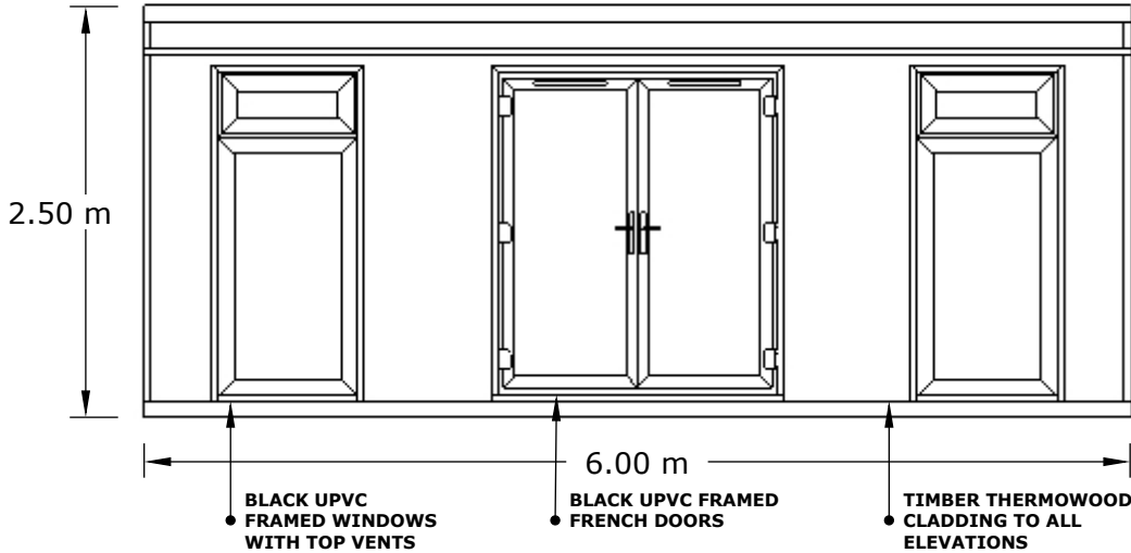
REAR ELEVATION
