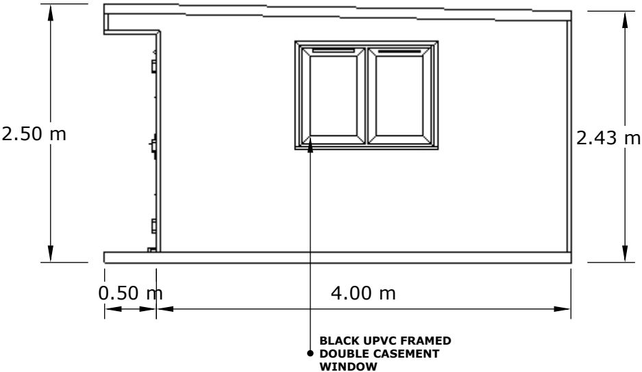
LEFT ELEVATION
