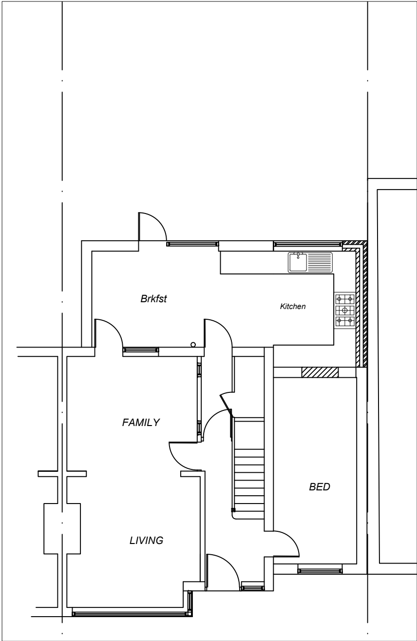
PROP GROUND FLOOR
