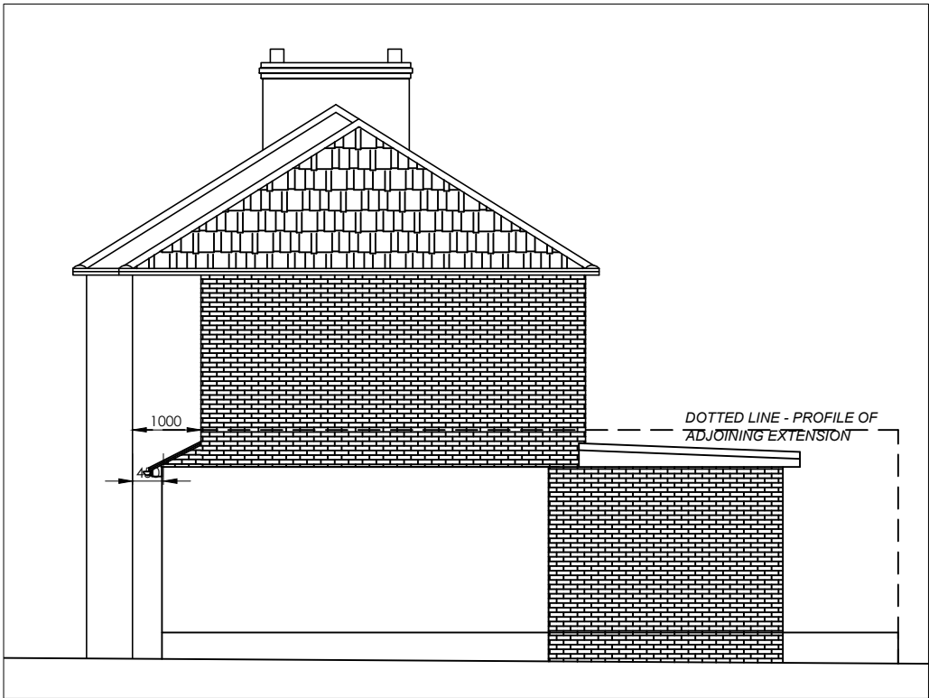
PROP SIDE ELEV (OTHER SIDE NOT AFFECTED)
