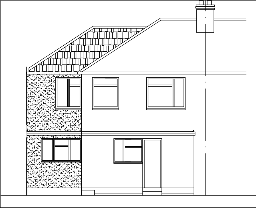
PROP REAR ELEV
