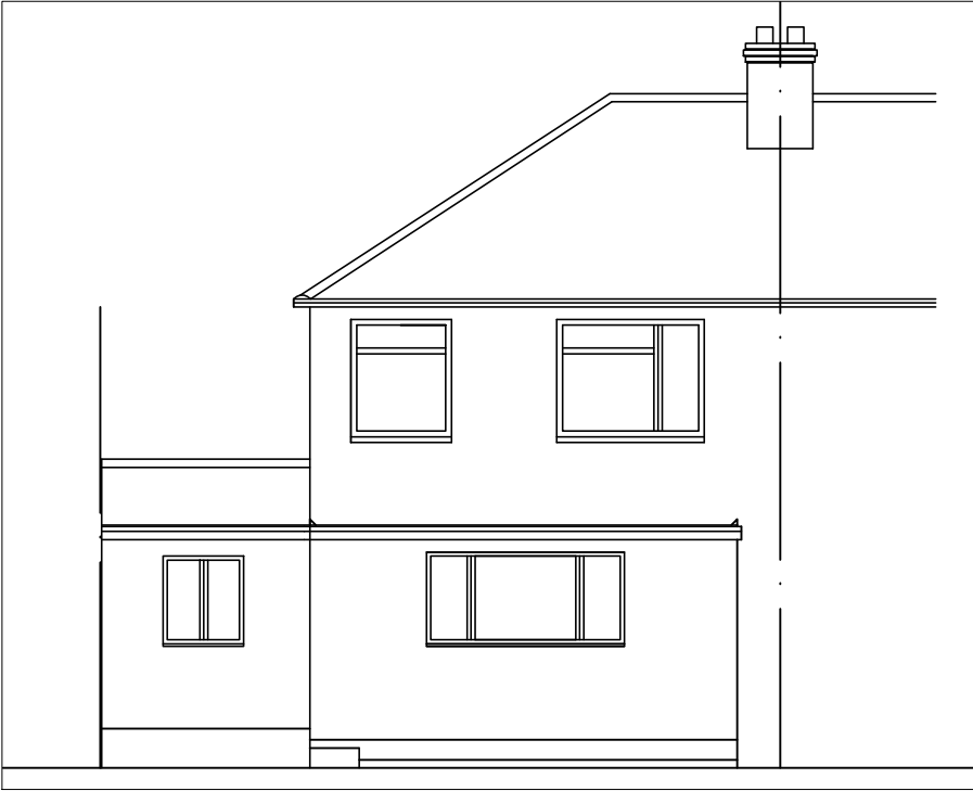
EXTG REAR ELEV
