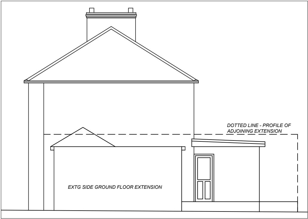
EXTG SIDE ELEV (OTHER SIDE NOT AFFECTED)
