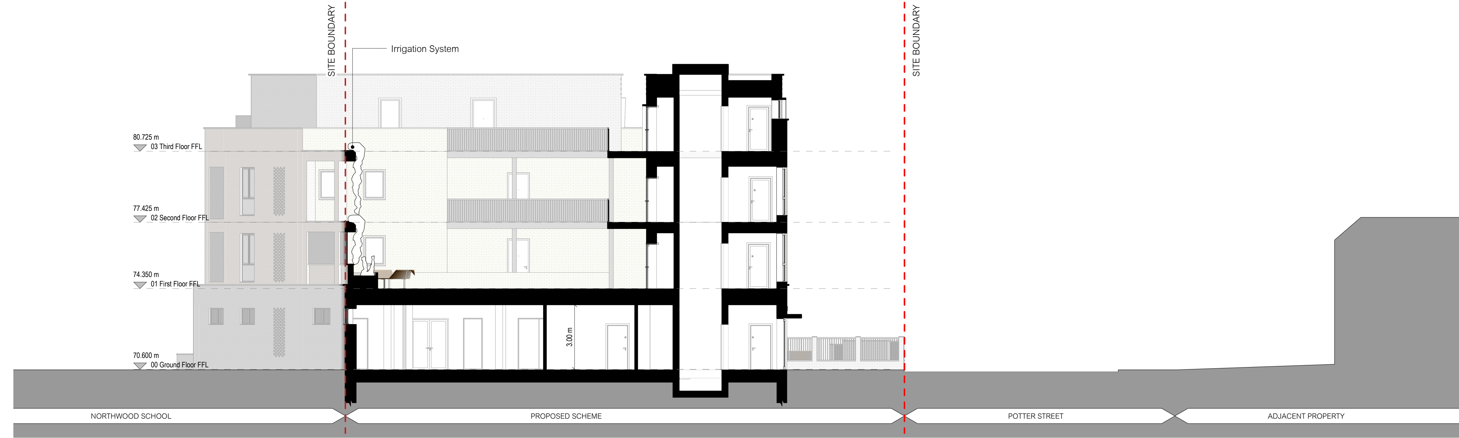
02 Proposed Section B-B' 1 : 100
