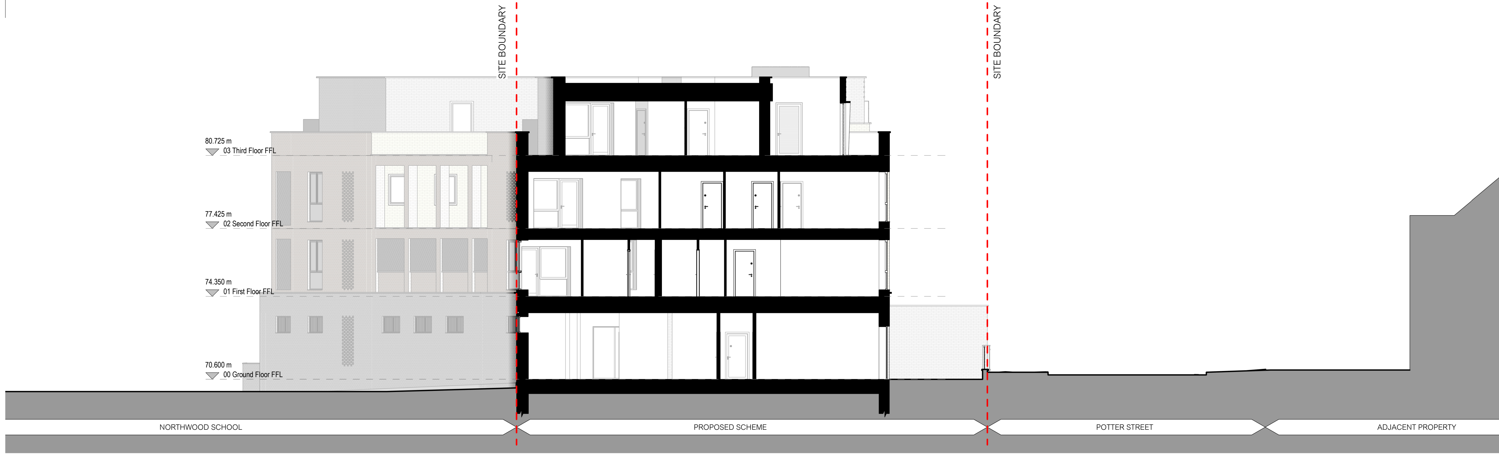
01 Proposed Section A-A' 1 : 100
