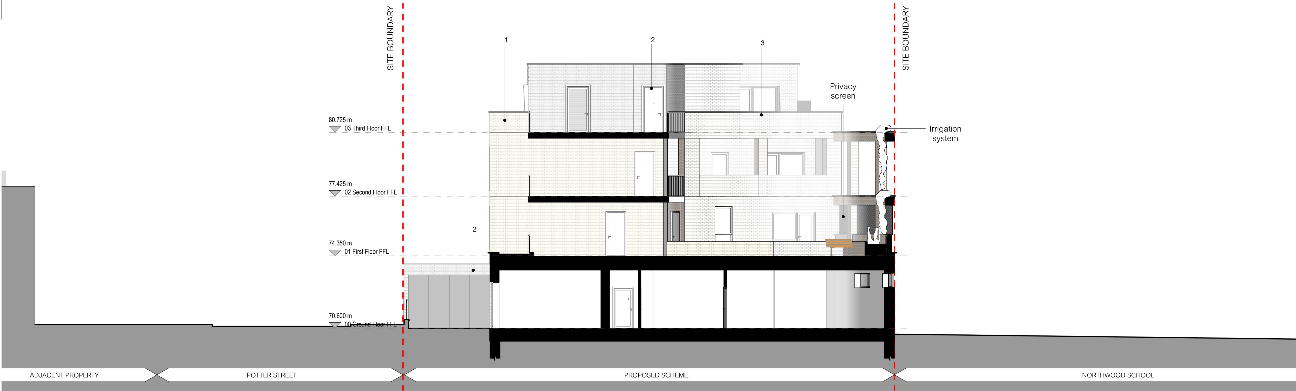
01 Proposed Elevation D-D' 1 : 100
