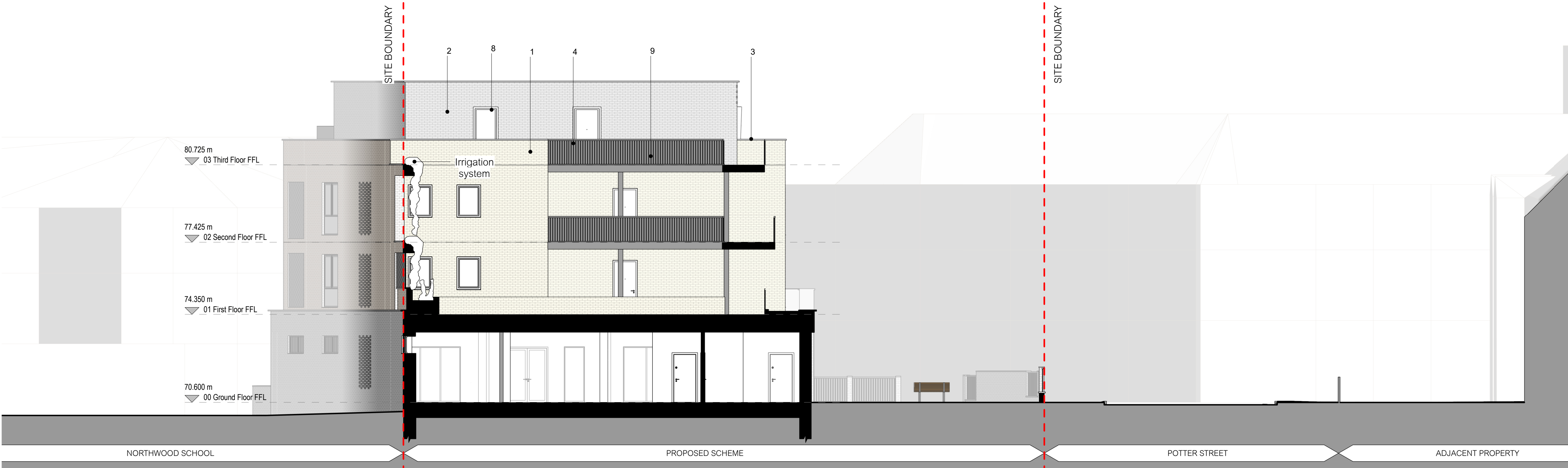
02 Proposed Elevation E-E' 1 : 100
