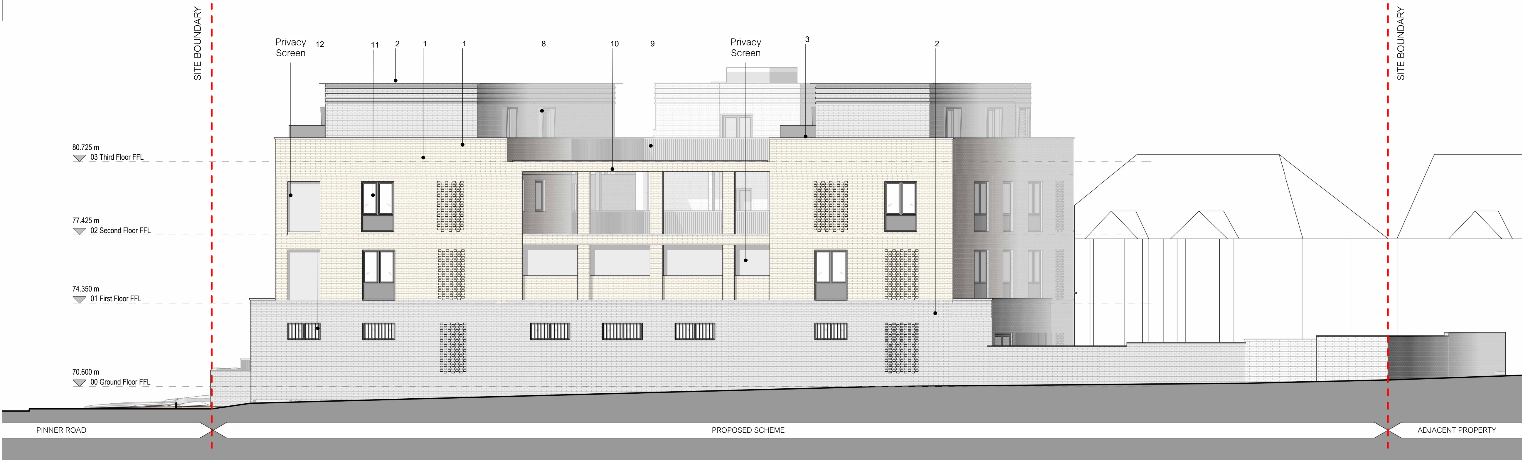
01 PROPOSED SOUTHEAST ELEVATION 1 : 100
