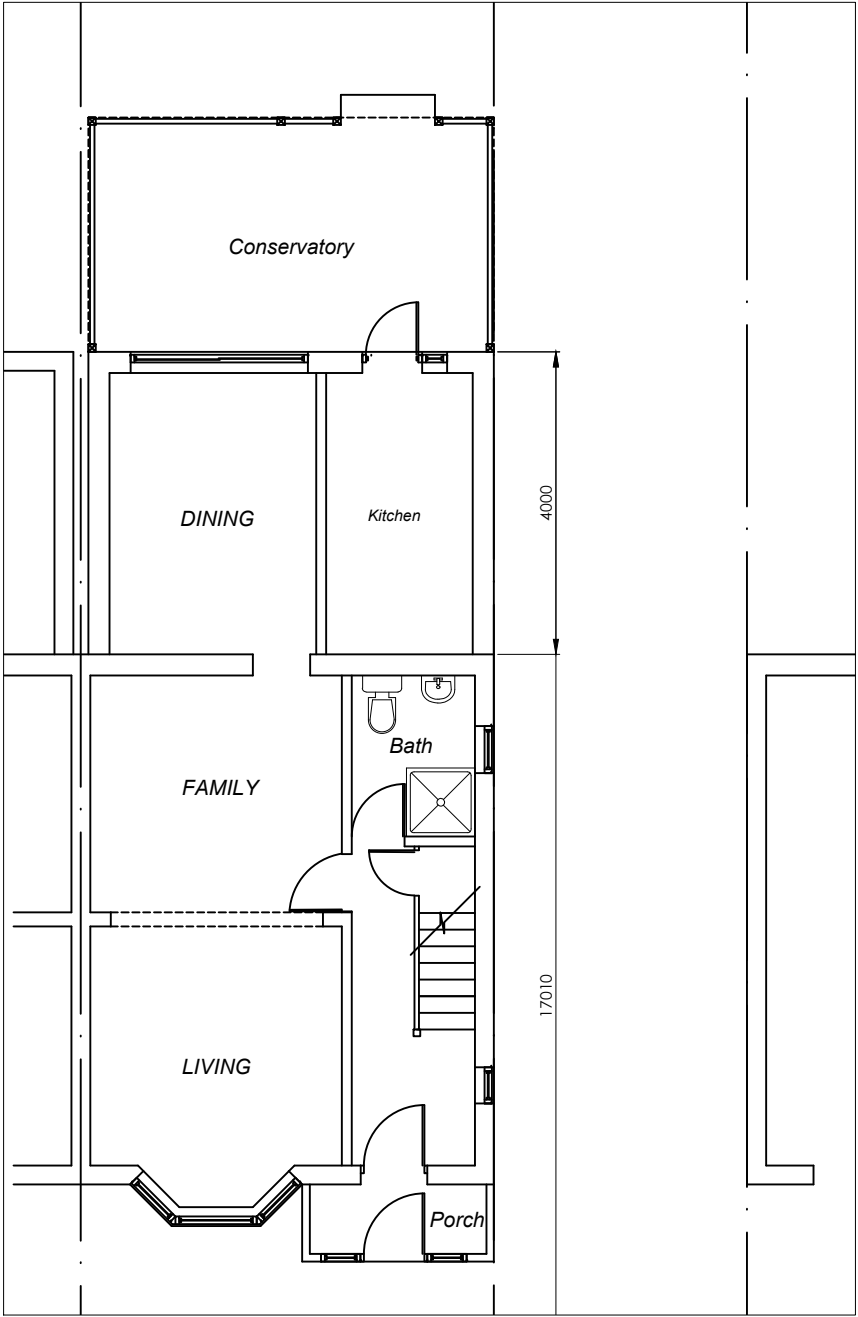
EXTG GROUND FLOOR
