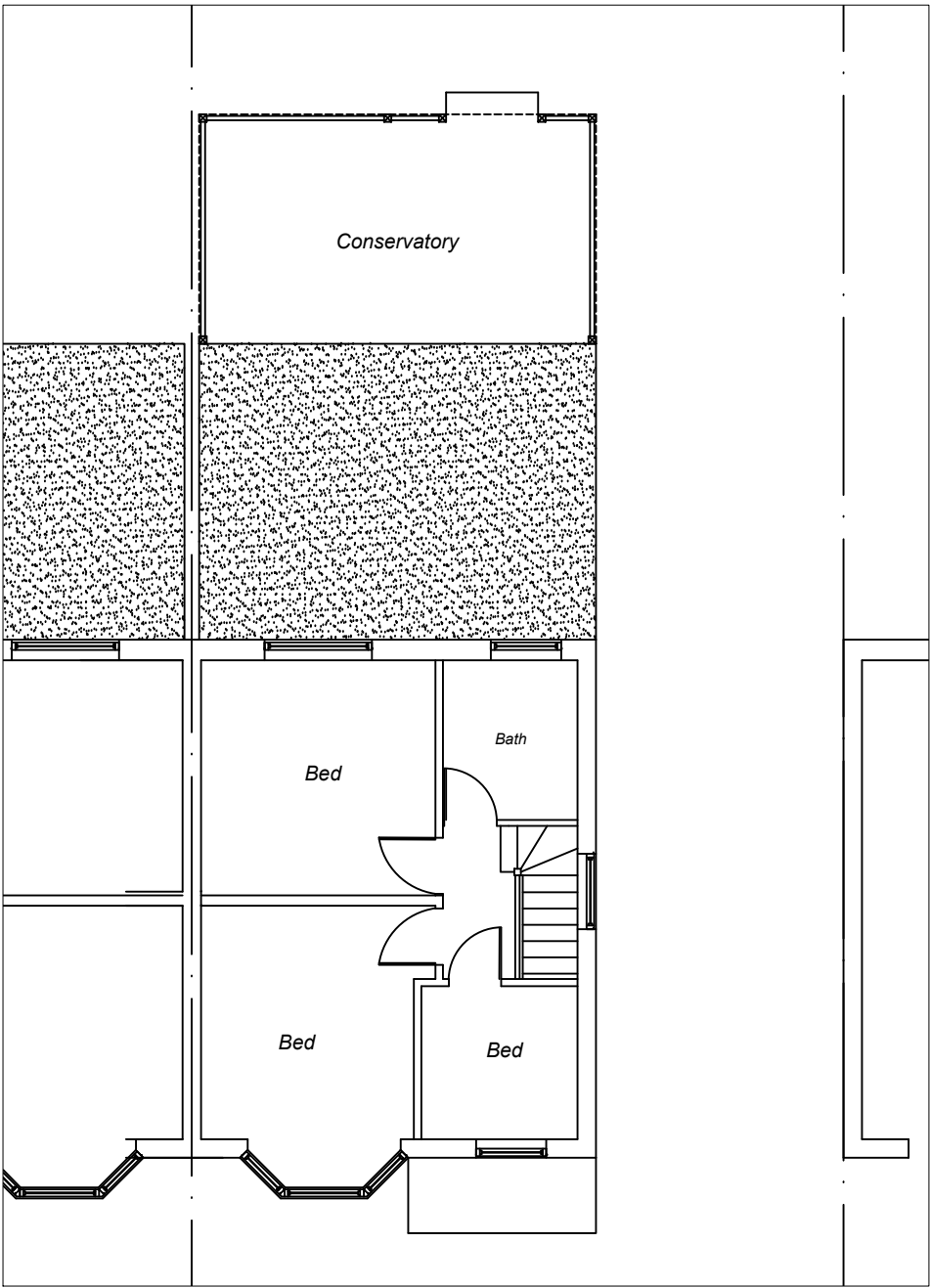
EXTG FIRST FLOOR
