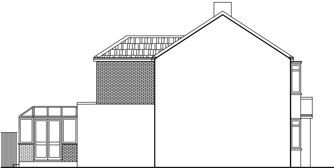
PROP OTHER SIDE ELEV
