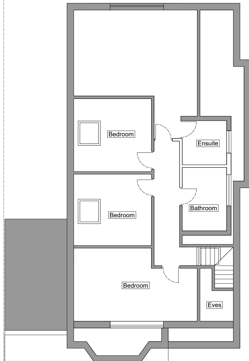
PROPOSED EXISTING FIRST FLOOR
