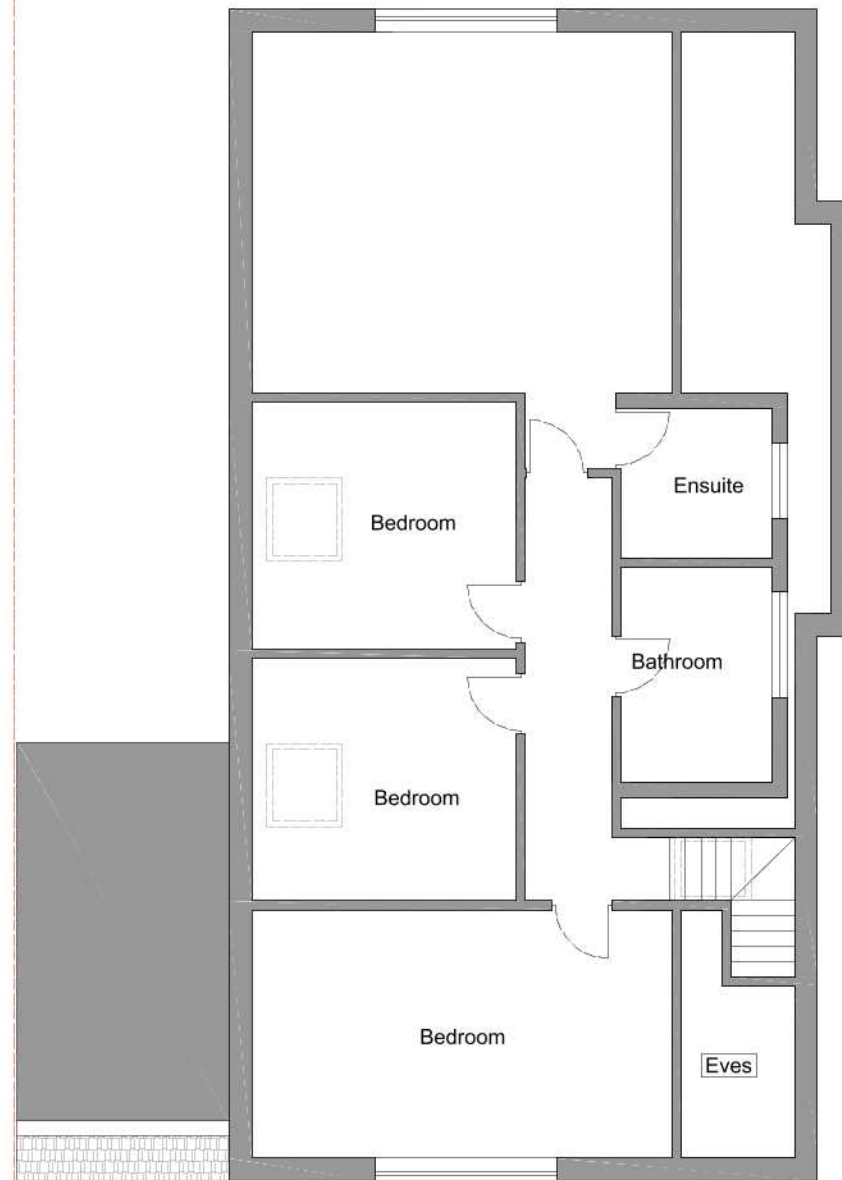
PROPOSED LOFT FLOOR PLAN
