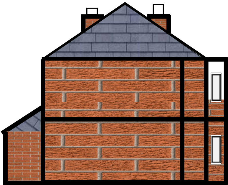
EXISTING LEFT SIDE ELEVATION (NORTH EAST SIDE)
