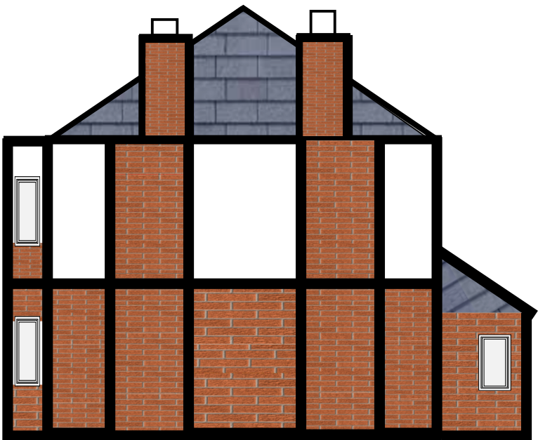
EXISTING RIGHT SIDE ELEVATION (NORTH WEST SIDE)
