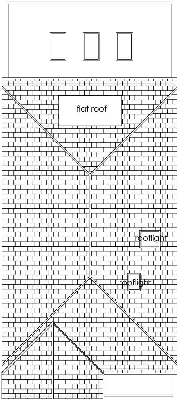
ROOF PLAN
