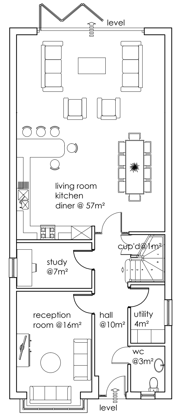
GROUND FLOOR PLAN GIA = 103m²
