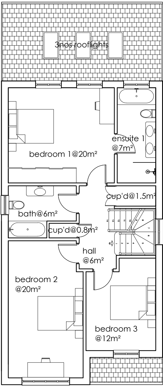
FIRST FLOOR PLAN GIA = 80m²
