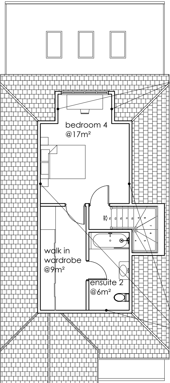
LOFT PLAN GIA = 36m² (taken at 1 at 1.8m height or greater)
