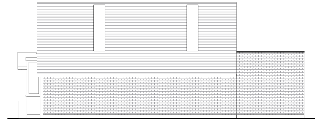
1 EX-20 SIDE ELEVATION Scale: 1/100
