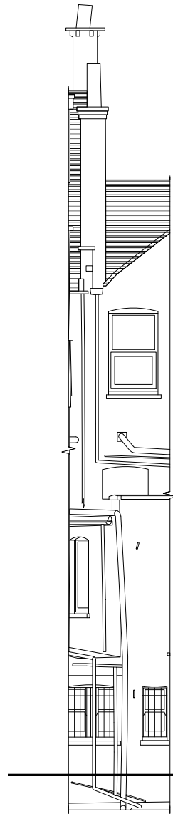
Existing Elevation 3
