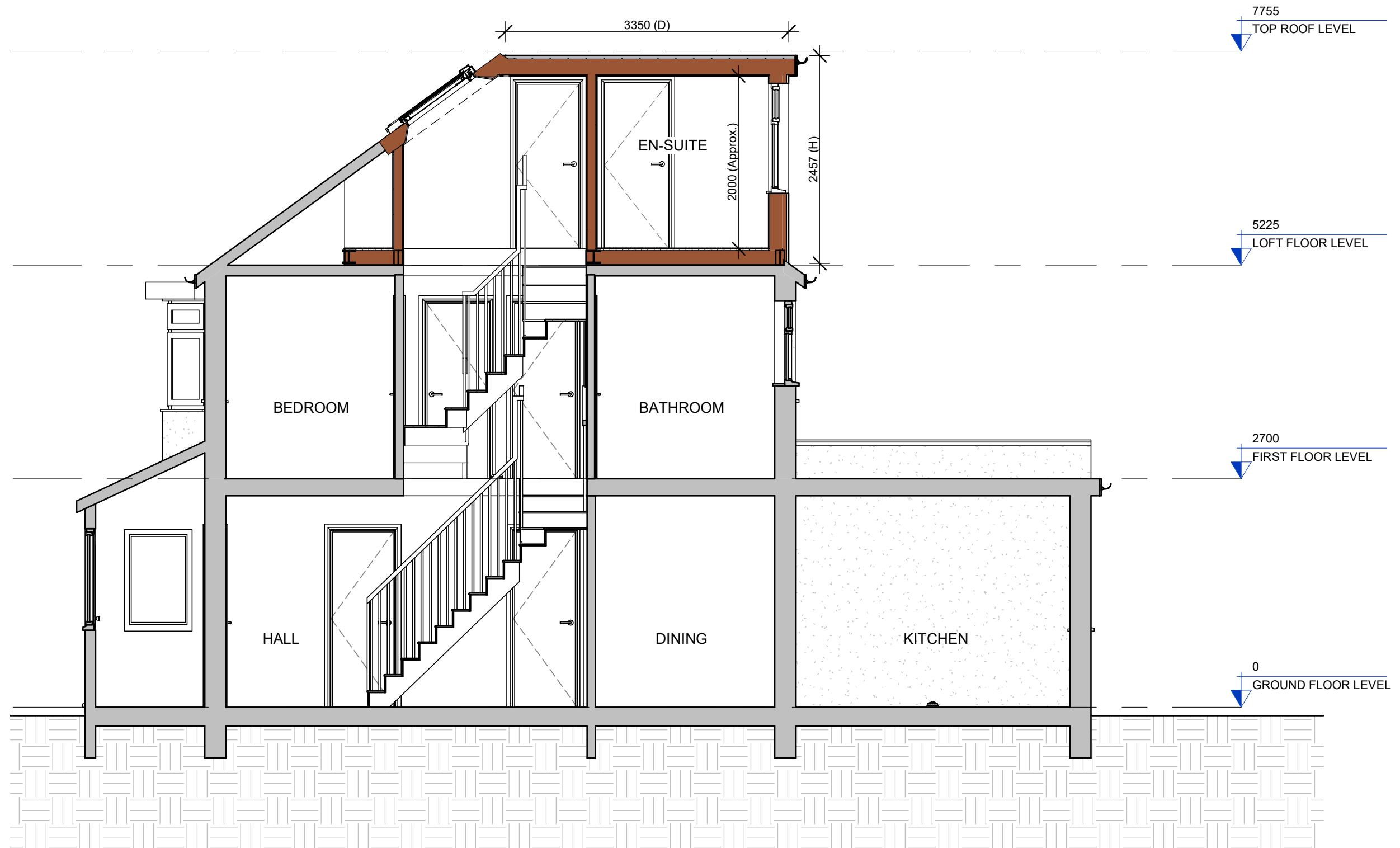
PP-PROPOSED SECTION A 1 : 50
