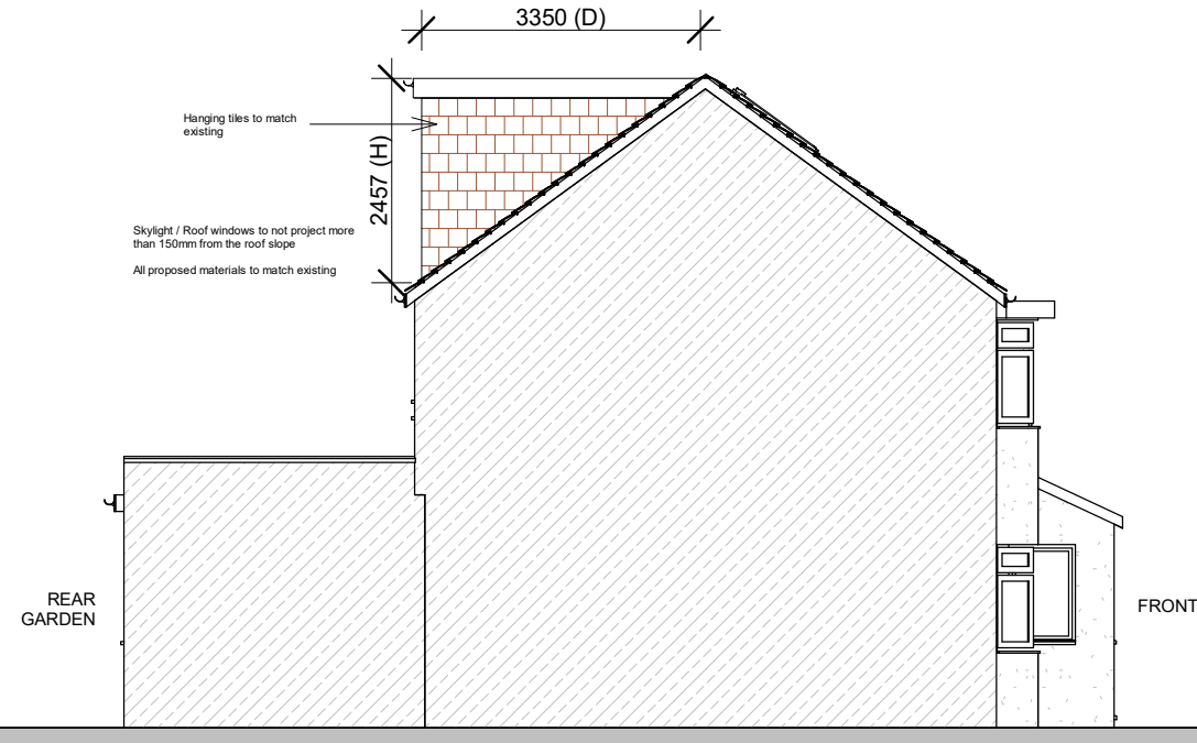
PP-PROPOSED LEFT SIDE ELEVATION 1 : 100
