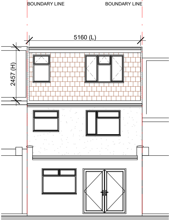
PP-PROPOSED FRONT ELEVATION 1 : 100
