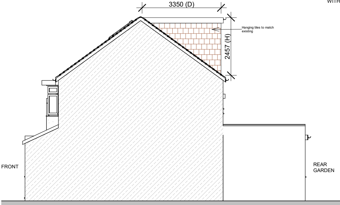
PP-PROPOSED RIGHT SIDE ELEVATION 1 : 100
