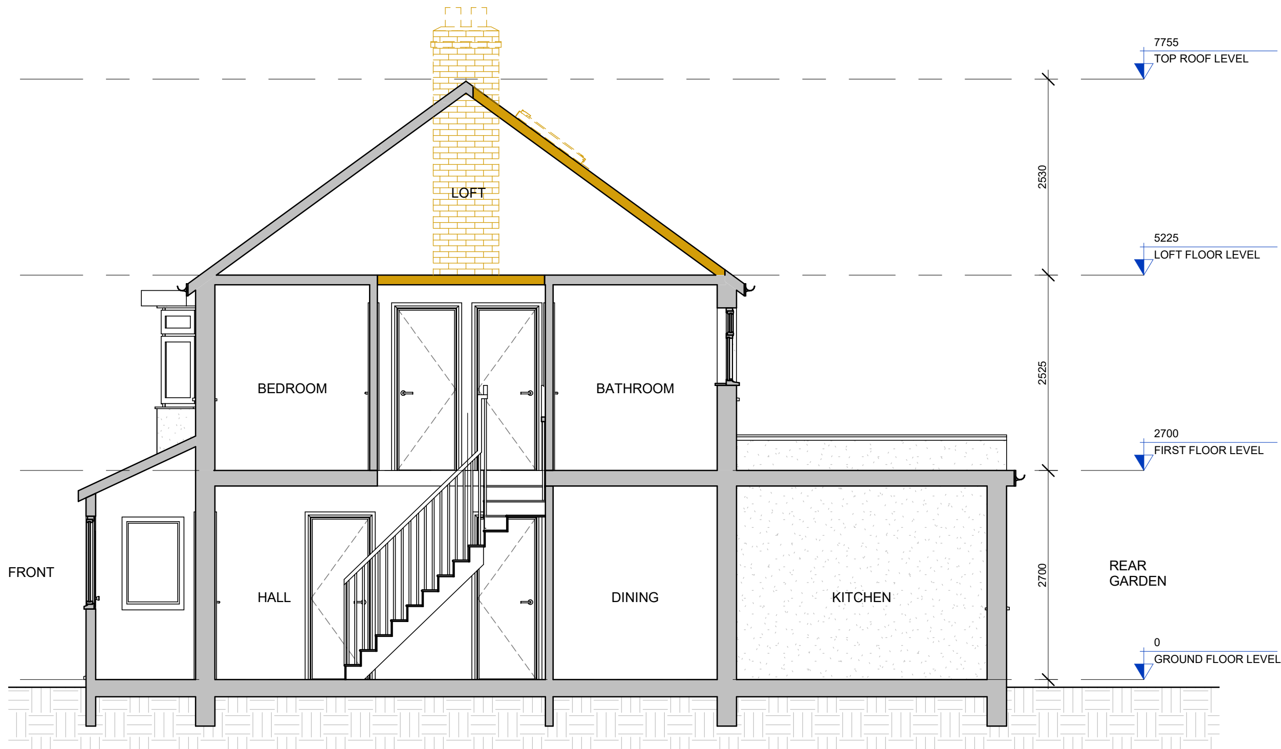
PP-EXISTING SECTION A 1 : 50
