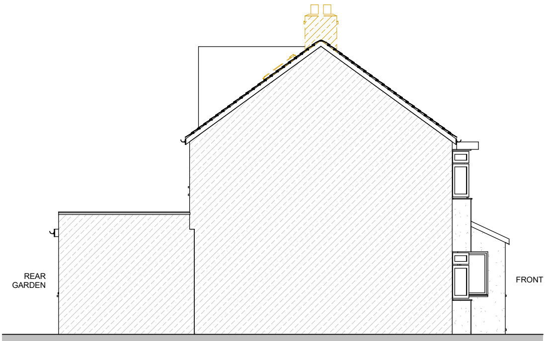
PP-EXISTING LEFT SIDE ELEVATION 1 : 100
