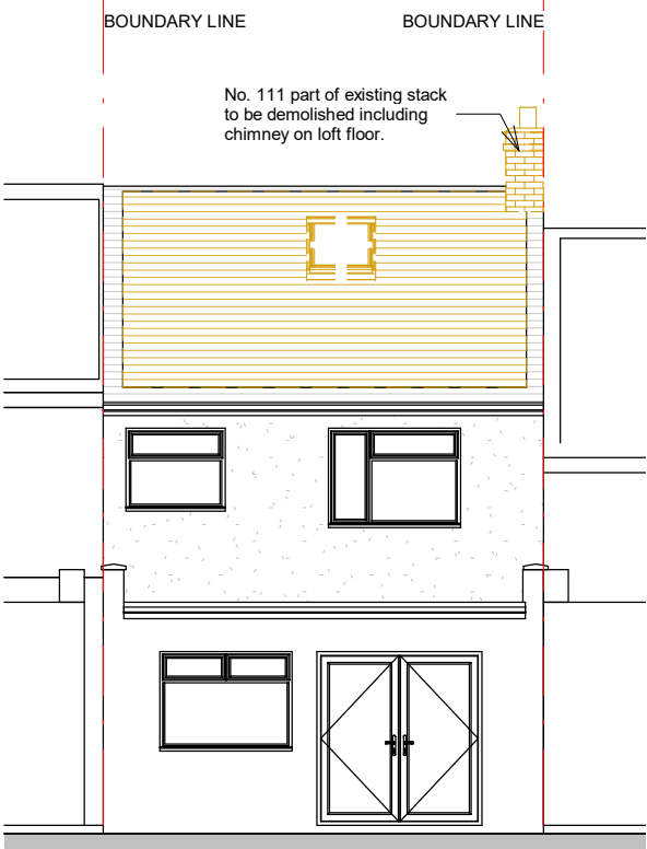
PP-EXISTING FRONT ELEVATION 1 : 100
