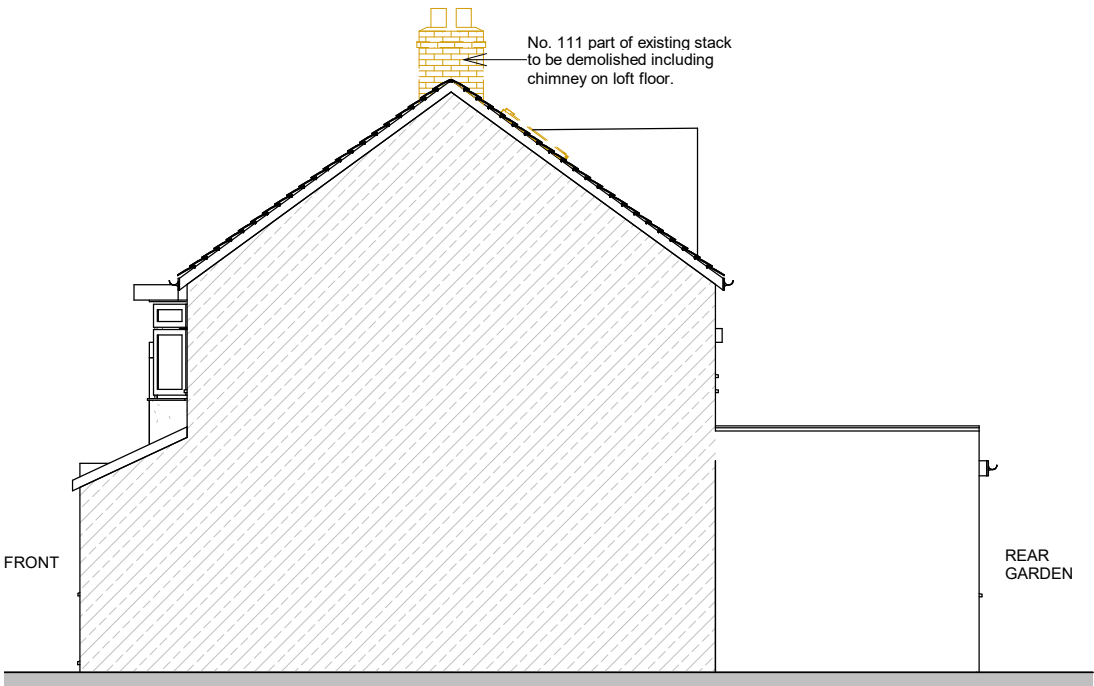
PP-EXISTING RIGHT SIDE ELEVATION 1 : 100
