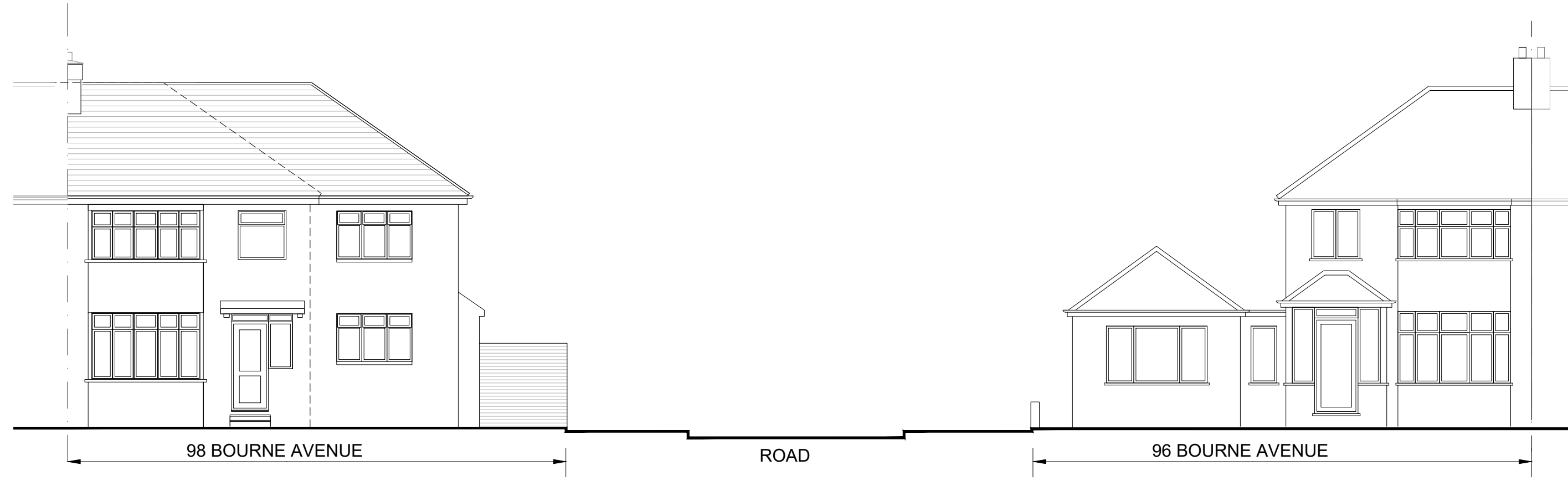
SOUTH ELEVATION 1:100
