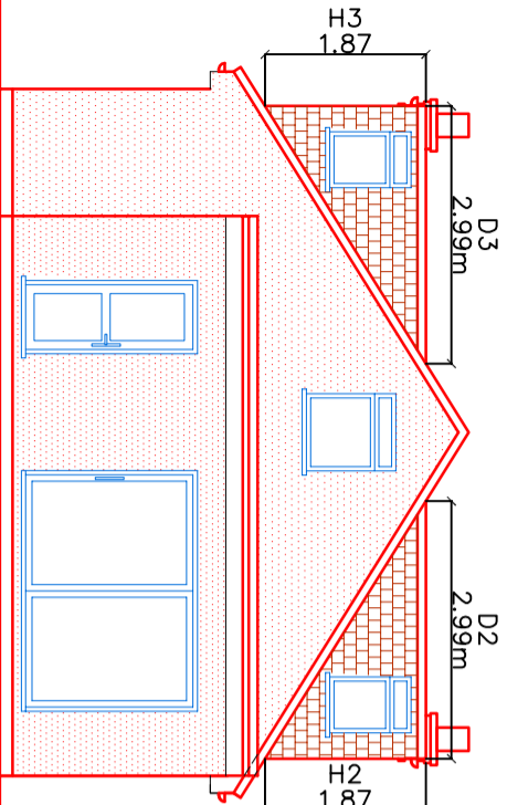
PROPOSED SIDE ELEVATION-1
