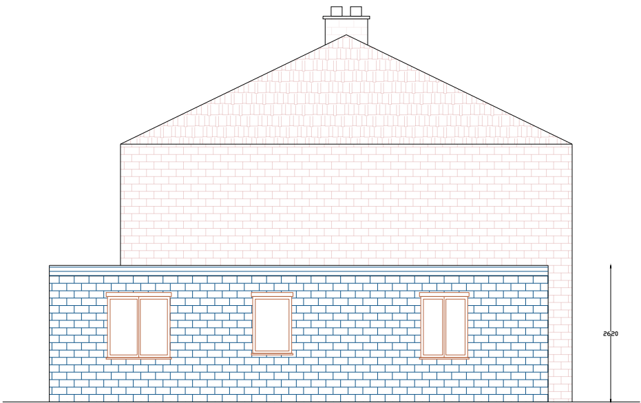
PROPOSED LEFT SIDE ELEVATION SCALE: 1:100
