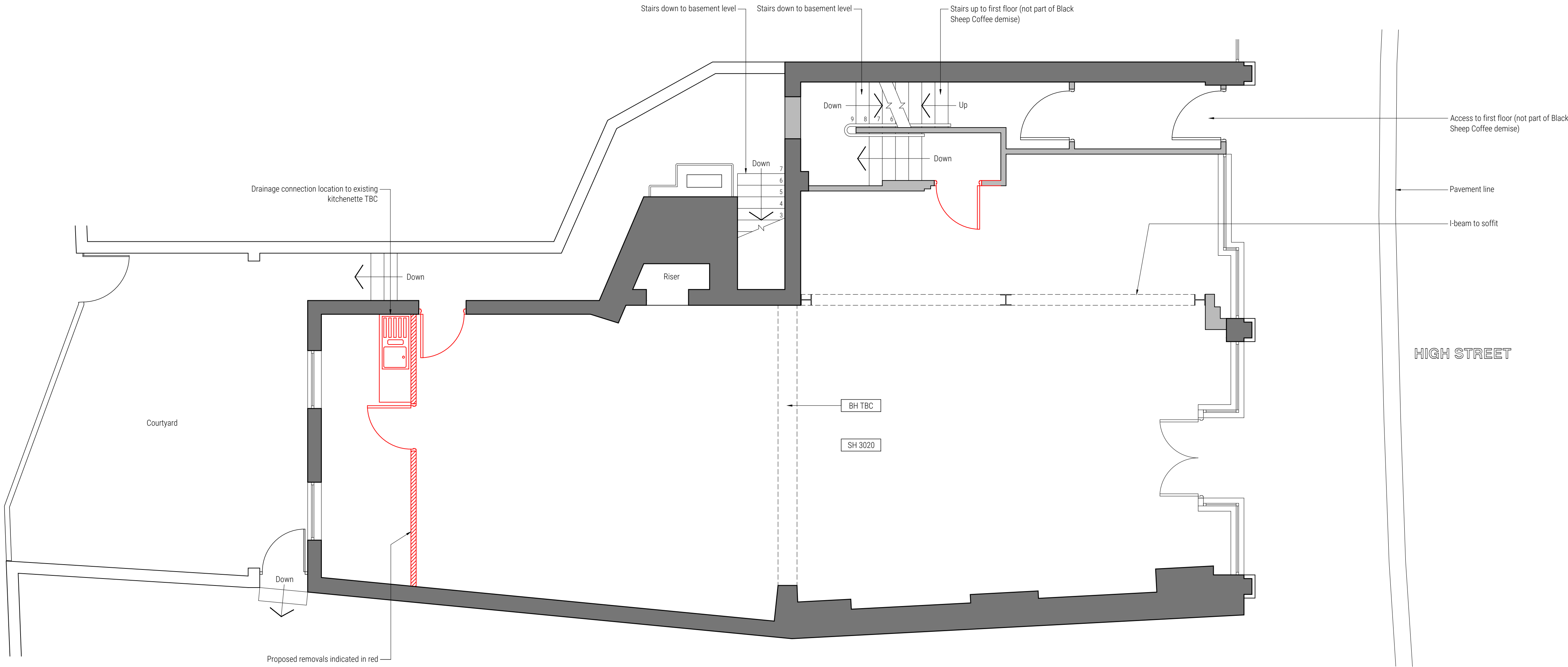
Existing Ground Floor General Arrangement Plan
